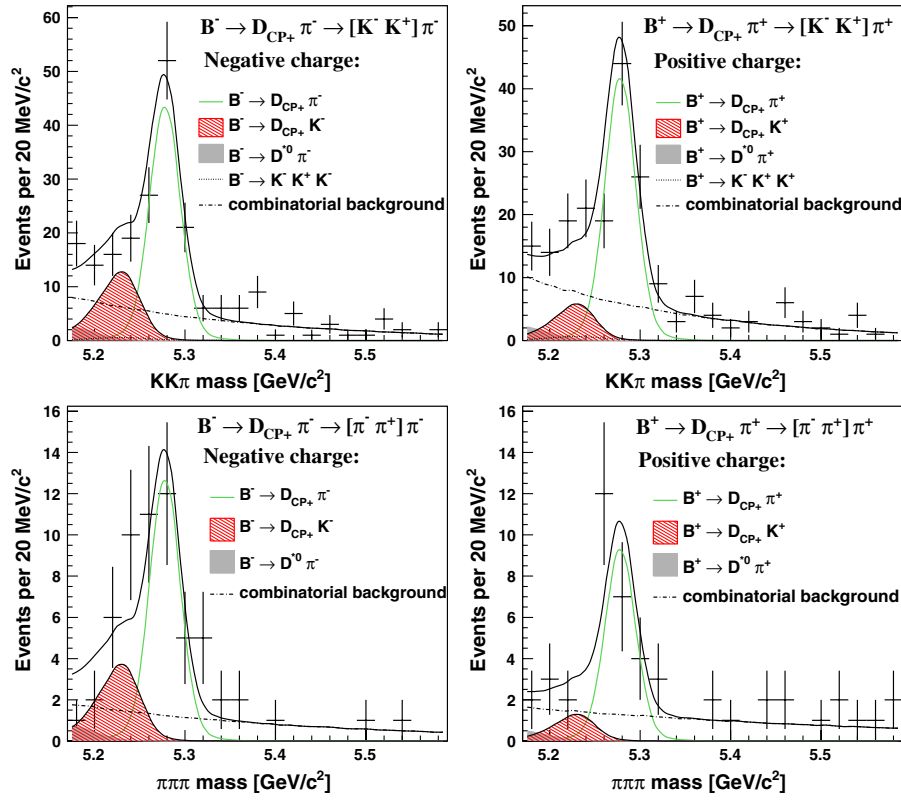
FIG. 3 (color online). Invariant mass distributions of B^- \rightarrow D_{CP+} \pi^- candidates for each reconstructed decay mode. The pion mass is assigned to the prompt track from the B decay. A requirement on the PID variable was applied to suppress the D\pi component and favor the DK component. The projections of the likelihood fit for each mode are overlaid. The p value for agreement of data with the fit is 0.95
