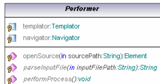
Figura 4.5 – Clase Performer
