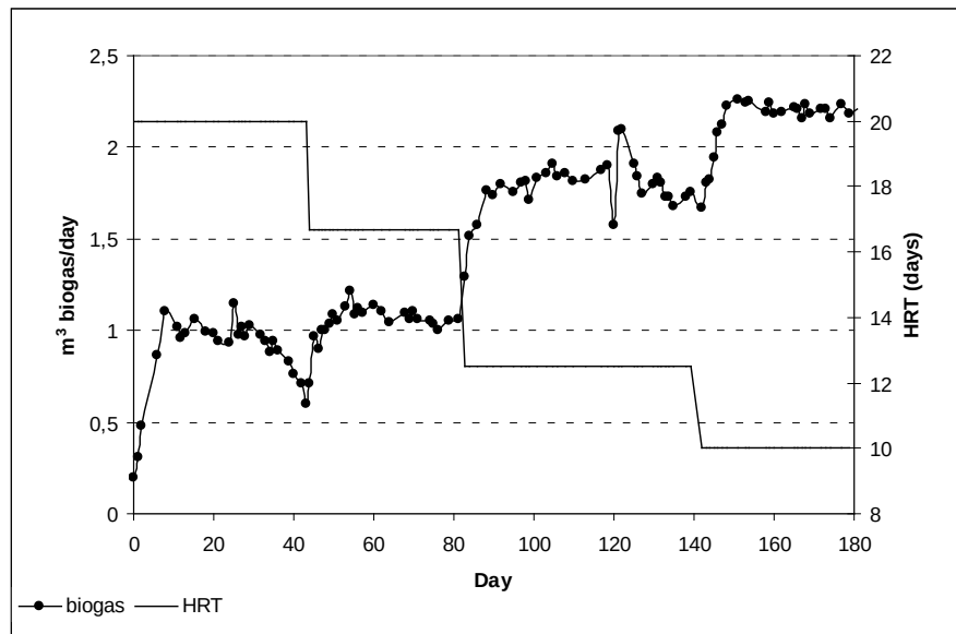
Figure 3- CSTR daily biogas production
