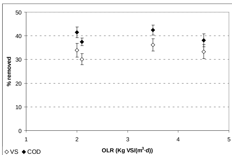
Figure 2- Removal percentage of VS and COD during CSTR operation
