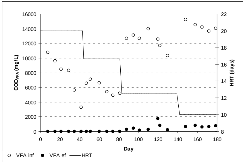
Figure 5- VFA in influent and effluent during CSTR operation
