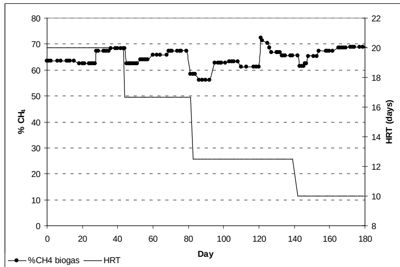
Figure 4- Biogas methane content during CSTR operation
