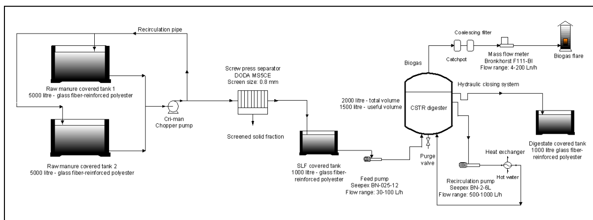
Figure 1- Scheme of the pilot installation
