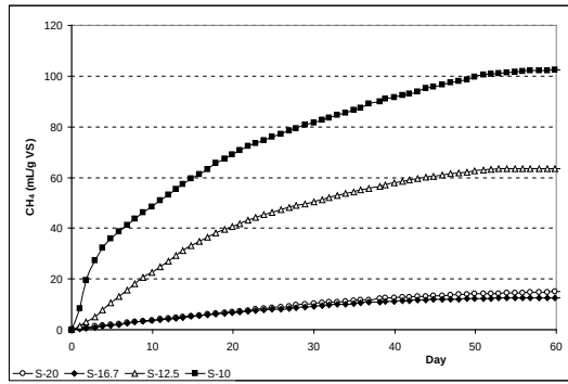
Figure 6- Methane cumulative (1) and daily specific methane yields (2) of digestate samples
