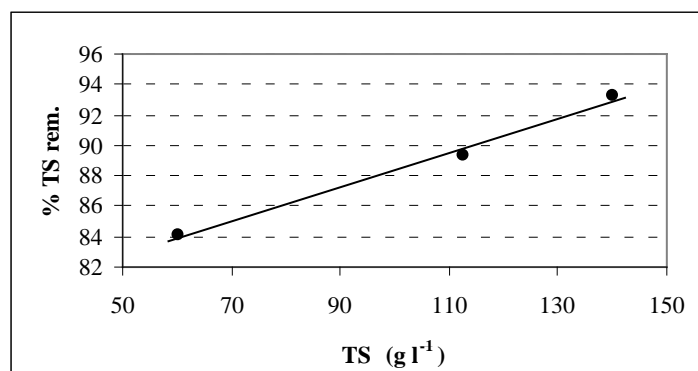
Fig. 2 - Correlation between sample concentration and removed percentage of TS.
