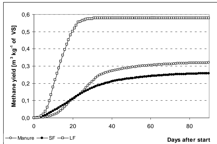
Fig. 3 - Specific methane productivity for manure, solid and liquid fractions.
