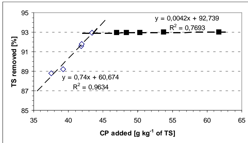
Fig. 1 - Percentage of TS removed in separation test using Raw Manure taken from Cow House (RMCH). Polymer added in form of solution. The dose is expressed as g of solid polymer added per kg of TS in manure.
