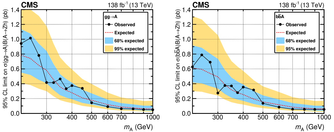
Figure 4. The expected and observed upper limits at 95% CL on the production cross section times branching fraction of the A \rightarrow Zh decay for gg \rightarrow A (left plot) and b\bar{b}A (right plot) processes as functions of m_A . The limits for the gg \rightarrow A ( b\bar{b}A ) process are derived with the rate of other process fixed to zero. The branching fraction of the h \rightarrow \tau\tau decay is set to the value predicted in the SM, \mathcal{B}(h \rightarrow \tau\tau) = 0.062 [54].
