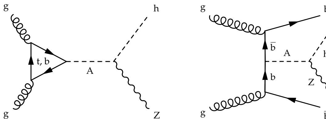
Figure 1. Feynman diagrams representing the production of the pseudoscalar A boson via gluon-gluon m_A - \tan \beta fusion (left) and associated production with a bottom quark-antiquark pair (right). In each case, the A boson decays to an SM-like h boson and a Z boson.
