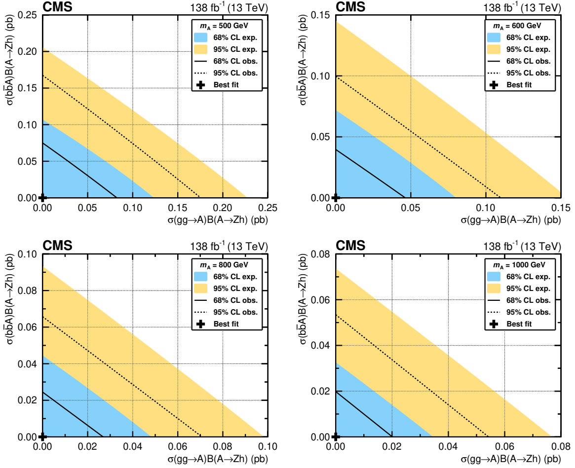
Figure 6. Same as figure 5 but for mass hypotheses of m_A = 500 (upper left plot), 600 (upper right plot), 800 (lower left plot) and 1000 GeV (lower right plot). The branching fraction of the h \rightarrow \tau\tau decay is set to the value predicted in the SM, \mathcal{B}(h \rightarrow \tau\tau) = 0.062 [54]. Computation of the best-fit point and determination of the observed and expected 68% and 95% CL contours are described in the text.
