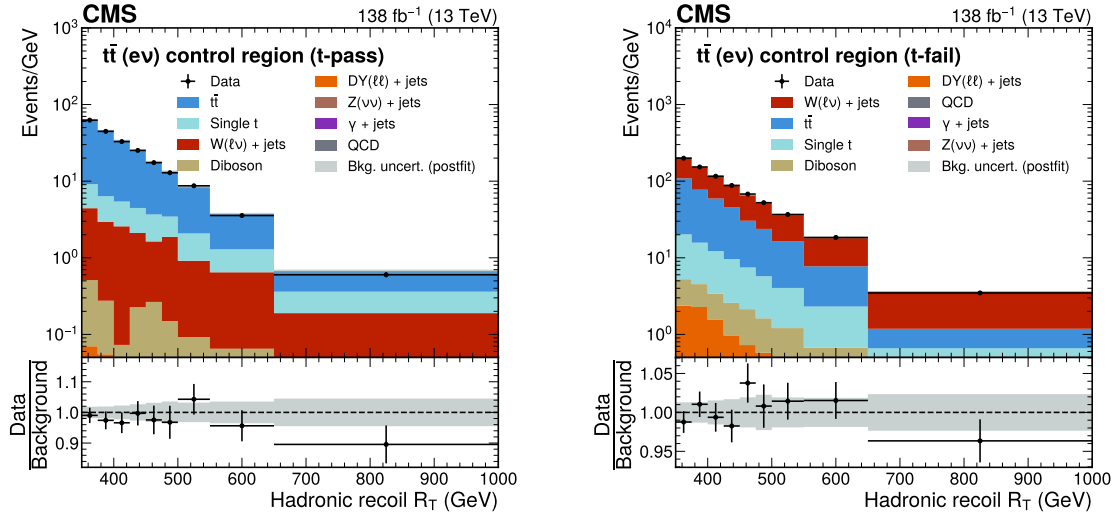
Figure 12. Postfit distributions of the magnitude of the hadronic recoil R_T in the t\bar{t}(e\nu) (t-pass) and t\bar{t}(e\nu) (t-fail) CRs after a fit of the background model to the data. The last bin of each distribution also contains events with R_T > 1000 GeV. The background processes are stacked together. The gray band represents the statistical and postfit systematic uncertainties in the predicted background yields after the fit.
