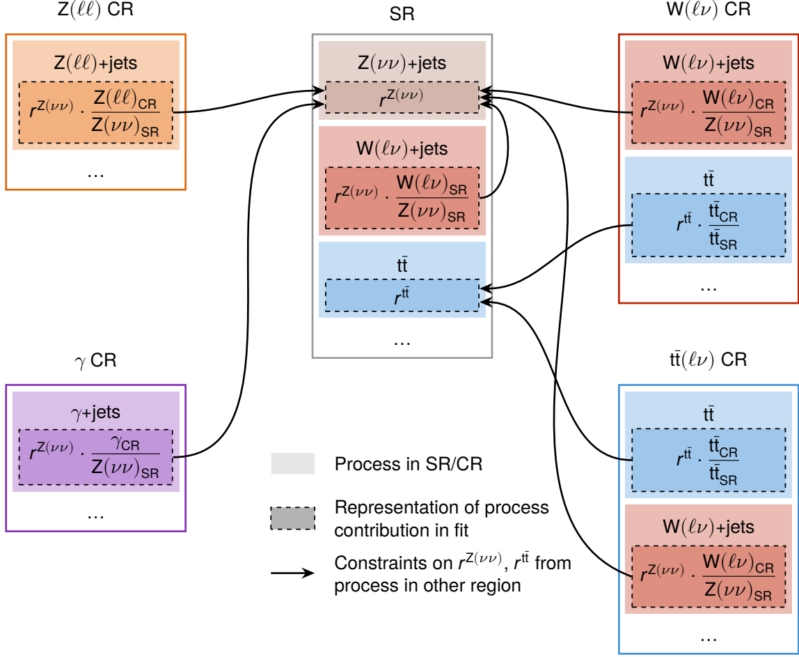
Figure 5. Statistical model used for the estimation of the major background processes for one bin of the R_T distribution. The contributions of Z(\nu\nu)+\text{jets} and t\bar{t} production in the SR are estimated with freely floating parameters r^{Z(\nu\nu)} and r^{t\bar{t}} . Constraints on Z(\nu\nu)+\text{jets} production are obtained by expressing similar processes in the SR and CRs as products of r^{Z(\nu\nu)} and a TF, obtained from simulation. Concerning t\bar{t} production, the t\bar{t} processes in the t\bar{t}(\ell\nu) and W(\ell\nu) CRs are expressed in terms of r^{t\bar{t}} and a TF. All processes not depicted in this illustration are estimated using simulated events. Regions containing charged leptons are included twice in this model, once for electrons and once for muons. The model is implemented for the t-pass and t-fail regions separately.
