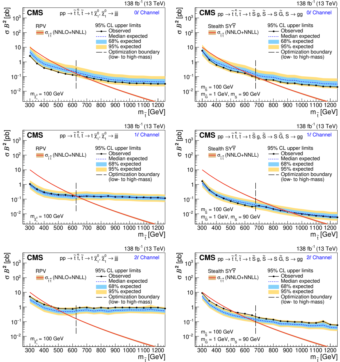
Figure 6. The 95% CL upper limit on \sigma_{\tilde{t}\tilde{t}} for the RPV (left) and stealth SY \tilde{Y} (right) SUSY signal models as a function of m_{\tilde{t}} for the 0\ell channel (upper), 1\ell channel (middle), and 2\ell channel (lower), assuming 100% branching fraction to the considered \tilde{t} squark decay. The median expected limit is shown in the dashed blue line, with the 68 and 95% intervals shown in light-blue and yellow, respectively. The observed limit is shown in black. The vertical dashed line denotes the transition from the low- to high-mass optimization ABCD boundaries. Additionally, the theoretical cross section is shown in red with its uncertainty in light brown.
