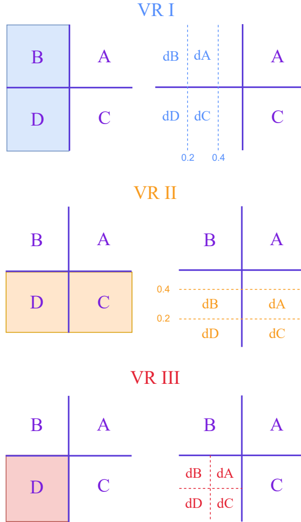
Figure 3. Illustrations of the three validation regions that are created by partitioning the S_{NN,1} - S_{NN,2} plane. VR I (VR II), shown in the upper (middle) row, is a division of the B and D ( C and D ) regions. VR III (lower row) is a division of the D region. Each VR is divided into four subregions (dB, dA, dC, dD) that are used to perform the validation of the nonclosure of the S_{NN,1} - S_{NN,2} plane. The subregion boundaries shown in the figure are the starting points of the stepping procedure explained in the text.
