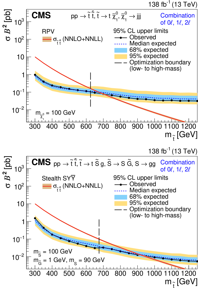
Figure 7. Observed and expected upper limits at 95% CL on \sigma_{\tilde{t}\tilde{t}} for the RPV (upper) and stealth SY \tilde{Y} (lower) SUSY signal models as functions of m_{\tilde{t}} for the combination of all three channels, assuming 100% branching fraction to the considered \tilde{t} squark decay. The median expected limit is shown in the dashed blue line, with the 68 and 95% intervals shown in light blue and yellow, respectively. The observed limit is shown in black. The vertical dashed line denotes the transition from the low- to high-mass optimization ABCD boundaries. Additionally, the theoretical cross section is shown in red with its uncertainty in light brown.
