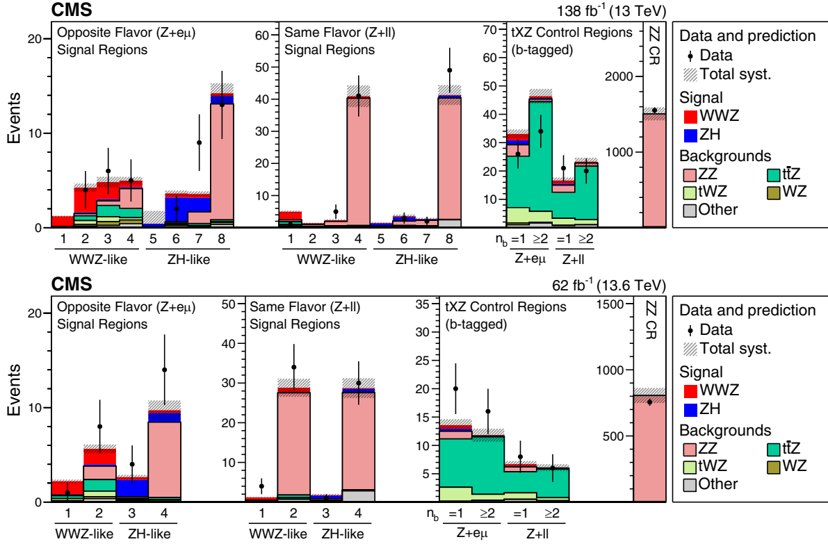
FIG. 2. Comparison of the numbers of observed to SM-predicted events for each of the bins included in the fit for Run 2 (upper row) and Run 3 (lower row). The SM expectations are shown before performing the fit. The horizontal axis legend also indicates WWZ -like and ZH -like bins defined based on whether the WWZ BDT score is higher or lower than the ZH score. The error bars on the data points represent the statistical uncertainties. The shaded bands represent the total contributions of the systematic uncertainties.
