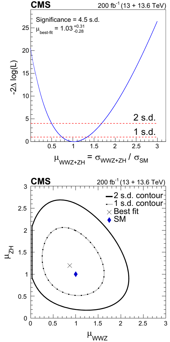
FIG. 3. Likelihood scans for the combined Run 2 and Run 3 datasets. Upper: one-dimensional likelihood scan as a function of the inclusive WWZ and ZH signal strength parameter ( \mu_{WWZ+ZH} ). Lower: two-dimensional scan as a function of the individual WWZ and ZH signal strength parameters. For the two-dimensional scan, the one and two standard deviation (s.d.) contours are indicated by the dotted and solid lines, respectively. The correlation coefficient is -0.23 . In the signal strengths reported here, the uncertainty of the predicted cross section is not included.
