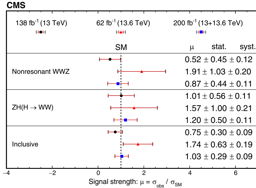
FIG. 4. Measured values of the WWZ , ZH , and inclusive signal strength parameters. Results are shown separately by run period as well as after combining the two datasets. The red error bars on the signal strengths represent the statistical uncertainty, and the black error bars represent the total uncertainty. In the signal strengths reported here, the uncertainty of the cross section prediction is not included.
