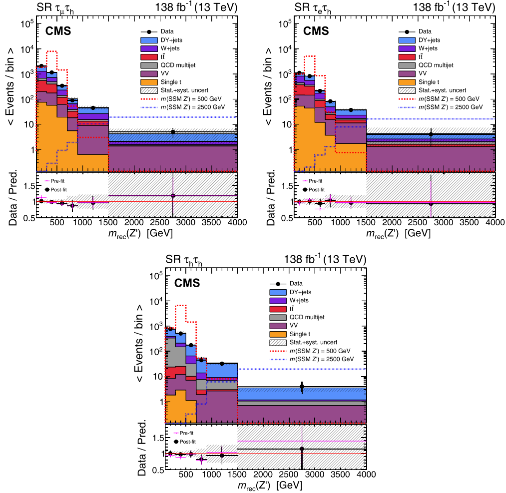
FIG. 2. Postfit reconstructed mass distributions for the (upper left) \tau_\mu\tau_h , (upper right) \tau_e\tau_h , and (lower) \tau_h\tau_h channel. The background contributions appear as stacked solid histograms, while the observed data are shown as black solid markers with error bars. Overflow counts are included in the last bin. The gray shadow band represents the statistical plus systematic uncertainty in the postfit background prediction. The ratio to the prefit background prediction is indicated in magenta markers in the ratio. The signal expectation is shown in lines for m_{Z'} of 500 GeV (red dashed) and 2500 GeV (blue dotted), normalized to 1850 and 0.131 pb, respectively.
