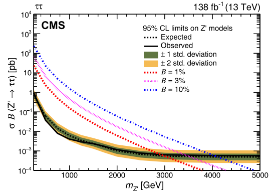
FIG. 4. Upper limits at 95% CL on \sigma\mathcal{B}(Z' \rightarrow \tau^+\tau^-) for the combination of all channels. The solid black line represents the observed limit, and the black dashed line with green and yellow bands depicts the expected limit with its one- and two-standard deviation uncertainties, respectively. The red dashed, magenta dotted, and blue dash-dotted lines represent the theoretical predictions for \mathcal{B}(Z' \rightarrow \tau^+\tau^-) = 1, 3 , and 10\% , respectively; 3\% is the value of \mathcal{B}(Z' \rightarrow \tau^+\tau^-) in the SSM. These assume that the \mathcal{B}(Z' \rightarrow \tau^+\tau^-) values are fixed for all m_{Z'} .
