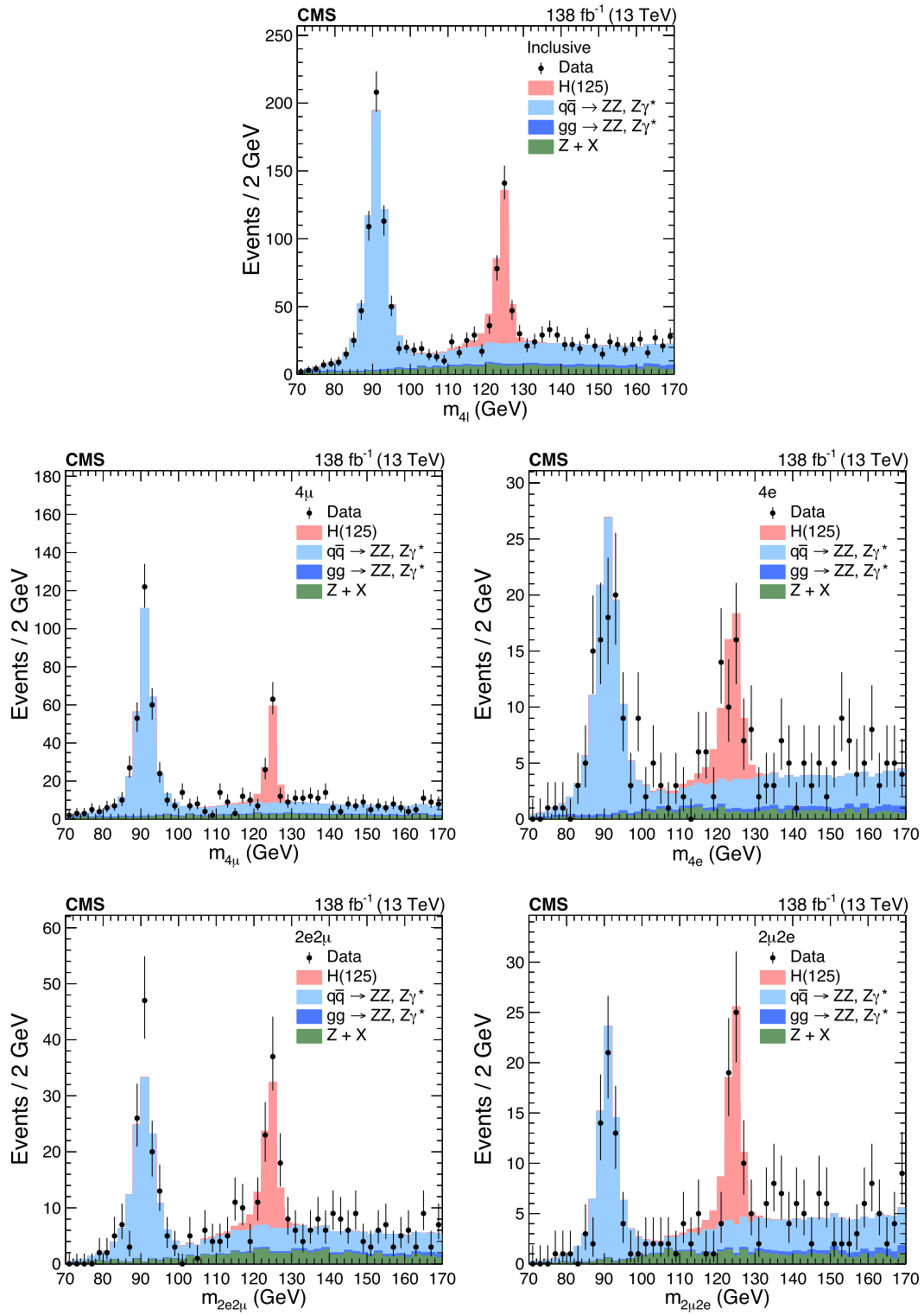
FIG. 1. The observed (points) and predicted (stacked histograms) m_{4\ell} distributions in the inclusive (upper), 4\mu (middle left), 4e (middle right), 2e2\mu (lower left) and 2\mu2e (lower right) final states, defined such that the first lepton pair is taken to be the one with the mass closest to the nominal Z boson mass. The predictions for the Higgs boson signal and the three main backgrounds are given by the different colors. The vertical bars on the points show the statistical uncertainties in the data.
