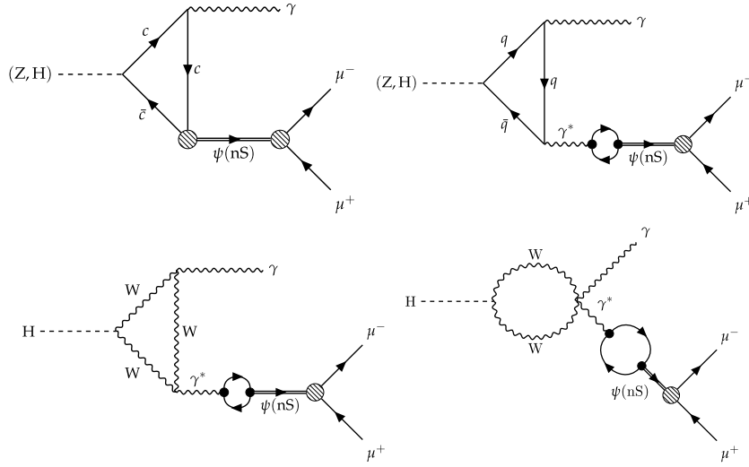
Fig. 1. Leading-order Feynman diagrams of Z and Higgs boson rare decays to J/\psi or \psi(2S) , and a photon, through the direct (upper top) and indirect (upper bottom, lower top, and lower bottom) processes. These four diagrams are considered as the signal of this analysis.
