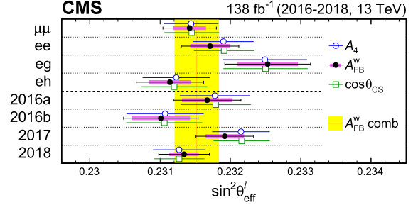
Fig. 10. Values of \sin^2\theta_{\text{eff}}^{\ell} measured with the A_{\text{FB}}^w , A_4 , and \cos\theta_{CS} fits, in each of the four channels using the full 2016–2018 sample (upper) and in each of the four data-taking periods combining the four channels (lower), always with the CT18Z PDF set. The “comb” band shows the result for all channels and runs combined. For the A_{\text{FB}}^w results, the magenta bands show the combined statistical and experimental systematic uncertainties, and the black bars represent the total uncertainties.
