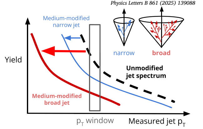
Fig. 1. Schematic diagram of the potential selection bias due to jet energy loss that may occur when selecting jets based on their p_T . Broader structures are expected to be more quenched (thicker red line and arrow), whereas narrower structures are expected to be quenched less (thinner blue line and arrow). Combined with the steeply falling jet p_T spectrum, this can lead to a preferential selection of narrow jets in a given jet p_T interval, as indicated by the vertical rectangular box. The dashed curve represents the jet p_T spectrum in the absence of medium-induced jet modifications.
