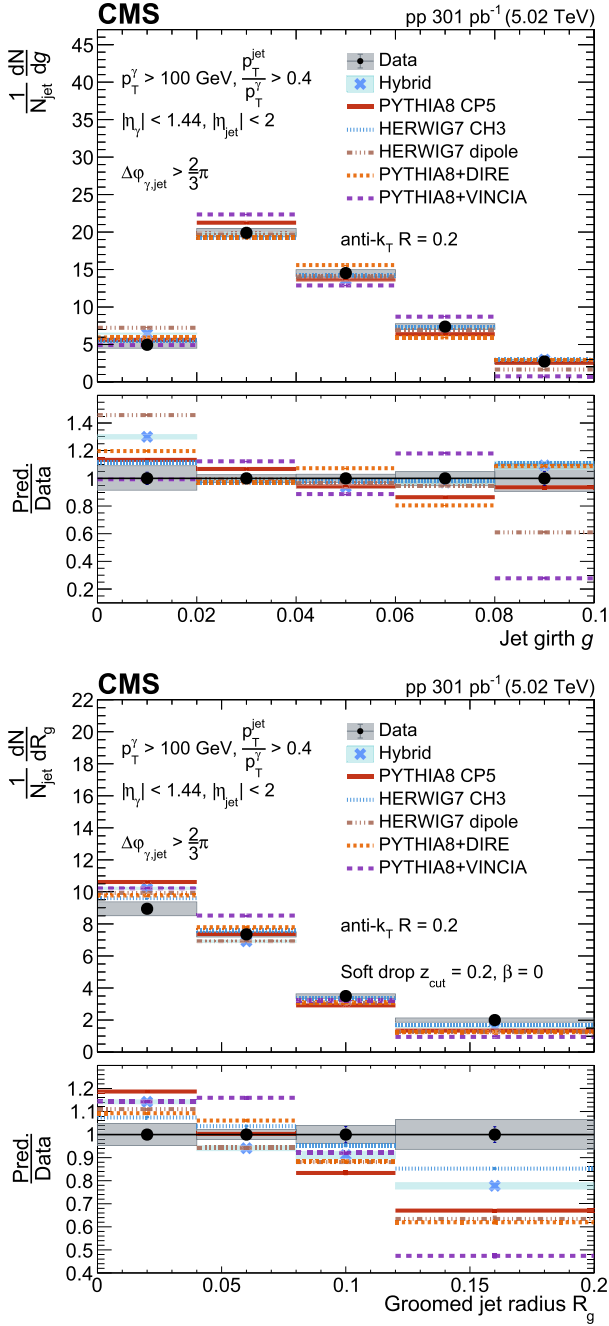
Fig. 2. Unfolded distributions of jet girth g (upper) and groomed jet radius R_g (lower) of photon-tagged jets in pp collisions for x_{\gamma j} \equiv p_T^{\text{jet}}/p_T^{\gamma} > 0.4 . The upper panels show the comparison of the observable in p_{\gamma j} and predictions from simulated events. The lower panels show the corresponding ratios of the MC calculations and data. The bands represent the total uncertainties, whereas the vertical bars represent the statistical uncertainties.
