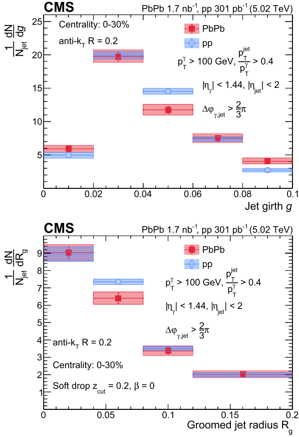
Fig. 4. Unfolded distributions of jet girth g (upper) and groomed jet radius R_g (lower) of photon-tagged jets in PbPb and pp collisions for x_{\gamma j} \equiv p_T^{\text{jet}}/p_T^{\gamma} > 0.4 (selecting both more and less quenched jets). The bands represent the total uncertainties, whereas the vertical bars represent the statistical uncertainties.
