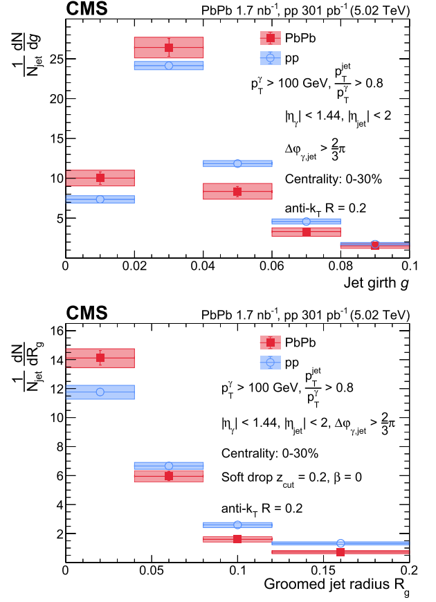
Fig. 5. Unfolded distributions of jet girth g (upper) and groomed jet radius R_g (lower) of photon-tagged jets in PbPb and pp collisions for x_{\gamma j} \equiv p_T^{\text{jet}}/p_T^{\gamma} > 0.8 (selecting less quenched jets). The bands represent the total uncertainties, whereas the vertical bars represent the statistical uncertainties.
