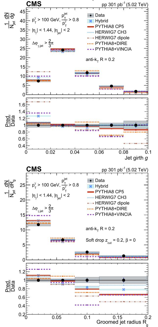
Fig. 3. Unfolded distributions of jet girth g (upper) and groomed jet radius R_g (lower) of photon-tagged jets in pp collisions for x_{\gamma j} \equiv p_T^{\text{jet}}/p_T^{\gamma} > 0.8 . The upper panels show the comparison of the observable in p_{\gamma j} and predictions from simulated events. The lower panels show the corresponding ratios of the MC calculations and data. The bands represent the total experimental uncertainties, whereas the vertical bars represent the statistical uncertainties.
