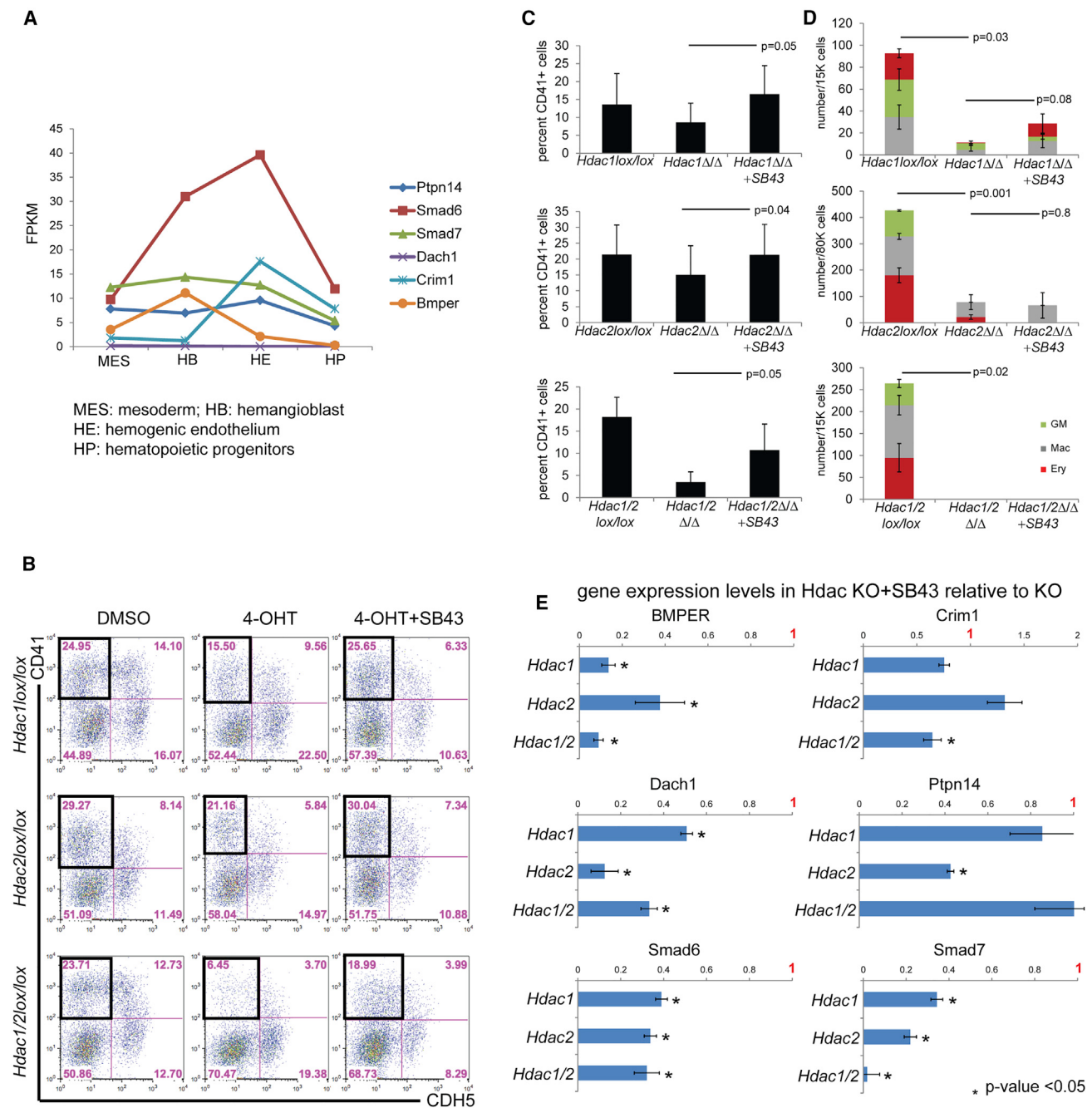
Figure 6. SB43 Treatment Increases Hematopoiesis
