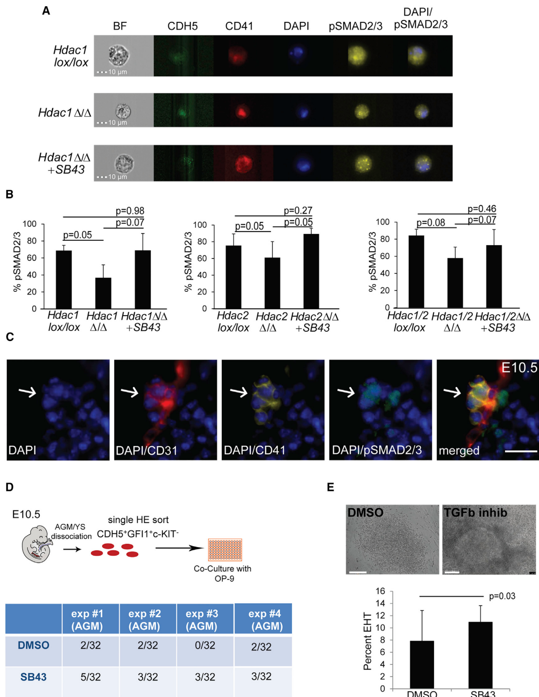
Figure 7. SB43 Treatment Increases TGF- \beta Signaling in Hdac1 and/or Hdac2 KO HE
