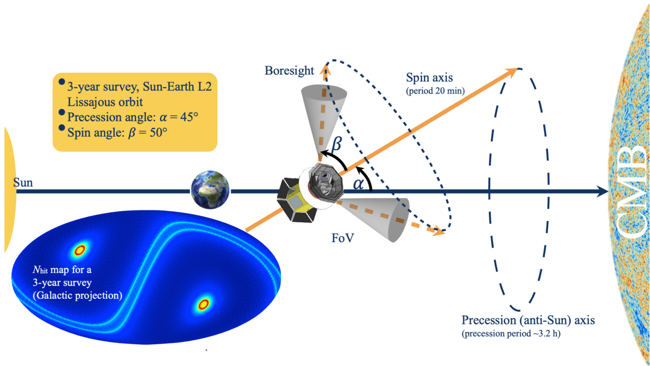
Figure 8. Visual summary of LiteBIRD scan strategy, which results from the combination of spin around the major axis of the spacecraft and precession of the spin axis around the anti-Sun direction. In the bottom left the expected hit-map for the whole duration of the mission (3 years) resulting from the baseline scan strategy (combined for all detectors). We can observe the high level of uniformity across most of the sky. Details of the size of the field-of-view (FoV) for all three telescopes can be found in Section 4.
