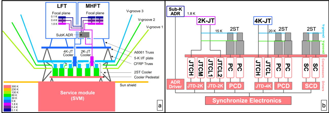
Figure 5. (a) Diagram depicting the thermal environment of the payload module (PLM). The Sun-shield delimits the service module (SVM) from the PLM and reduces the thermal loading on the PLM. A series of three V-grooves is employed in combination with two-stage Sterling coolers (2ST) to cool the PLM below 30 K. Active cooling (combination of Joule-Thomson (JT) and adiabatic demagnetization refrigerators) is used to set the temperature of the coldest stages all the way to the 100 mK required for the focal plane units (FPU). (b) Diagram of the cooling system. Figures are adapted from 46. Most acronyms are explained throughout the text, but here is a list of those that are not explained elsewhere: JTCH = JT compressor for high-pressure stage; JTCM = JT compressor for medium-pressure stage; JTCL = JT compressor for low-pressure stage; JTD = JT cooler driver; PC = precooler; PCD = precooler driver; SC = shield cooler; and SCD = shield cooler driver.
