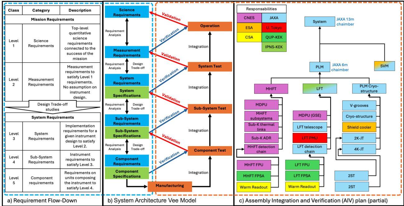
Figure 2. Simplified schematic of the requirements flow-down (a) and verification plan (c), based on systems engineering concepts (b). We highlight the connection between requirements and the validation and verification cycle at each stage of the system development. For more details on this topic, see 14.
