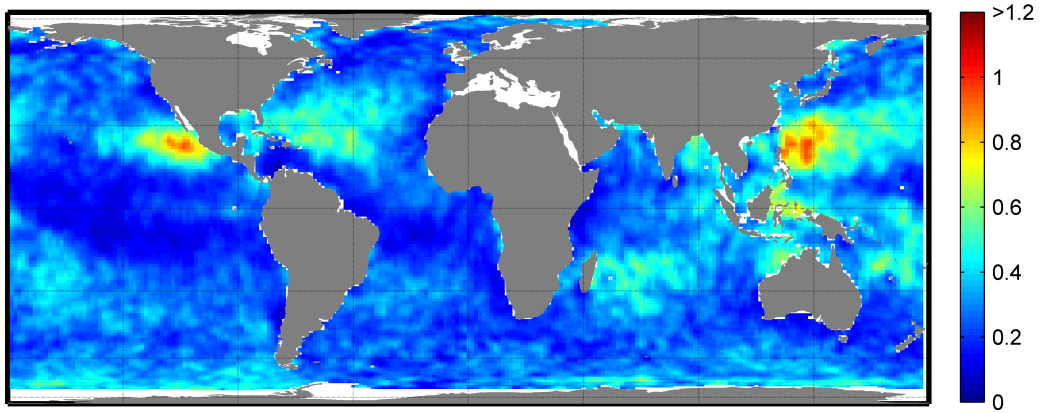
Figure 10: Spatial distribution of the percentage of outliers removed at each location within GOW domain, for a given confidence level \alpha = 0.0001 .
