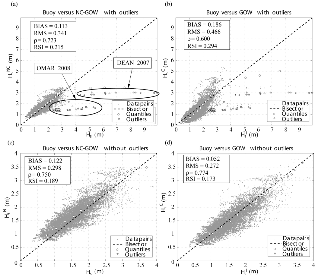
Figure 9: Scatter and quantile-quantile plots before (a, c) and after (b, d) the calibration process, without the outlier identification (a, b) and after the removal of the outliers (c, d). Outliers due to Dean and Omar hurricanes are outlined in panel a.
