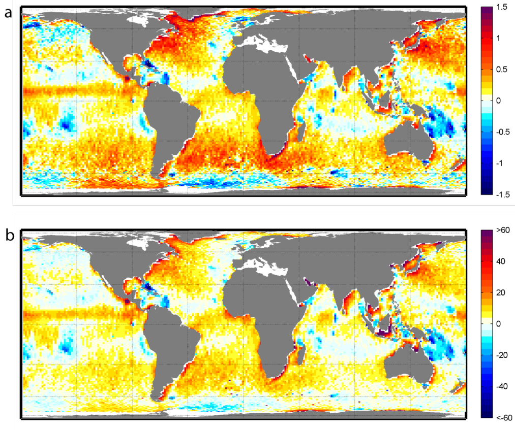
Figure 15: Absolute (a; GOW - NC-GOW ) and relative (b; [GOW - NC-GOW] / NC-GOW ) change in the 95 th percentile of significant wave height in the reanalysis data for the period from 2006 to 2008 after the calibration process. Calibration is computed with a training set of altimeter data from 1992 to 2005.
