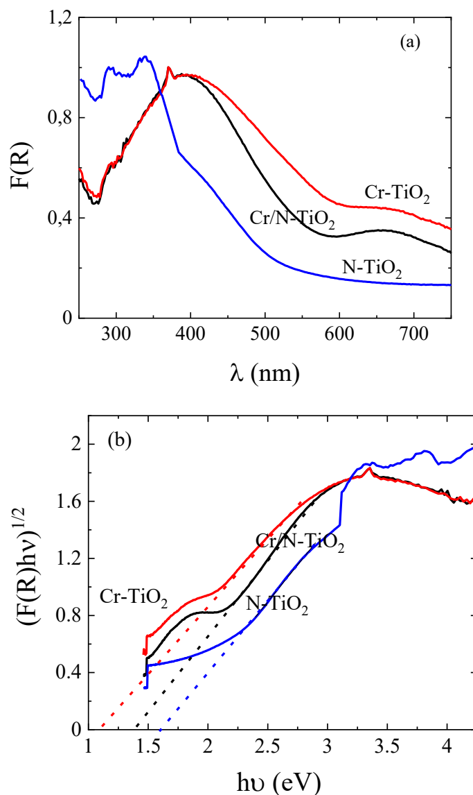
Figure 6: (a) UV-Vis spectra (Kubelka-Munk function F(R) versus wavelength, \lambda , and (b) Tauc plots ((F(R)h\nu)^{1/2}) versus h\nu for the doped TiO 2 nanoparticles.
