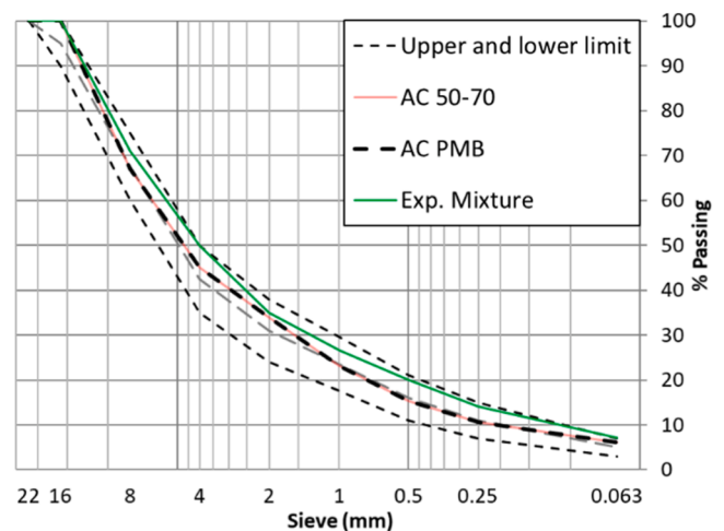
Fig. 2. Granulometric distribution.
