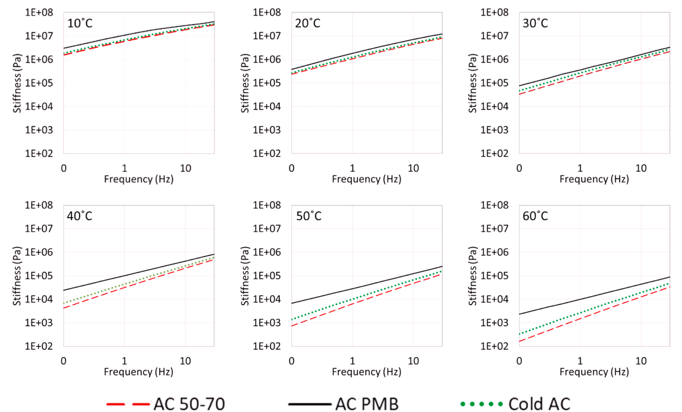
Fig. 4. DSR test results: stiffness.
