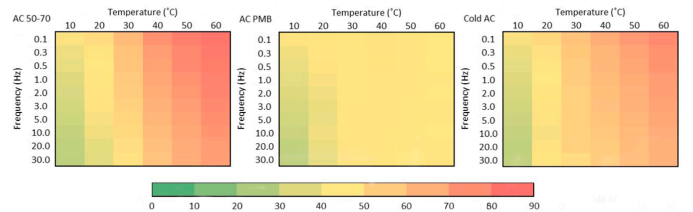
Fig. 5. Dynamic shear rheometer: phase angle.
