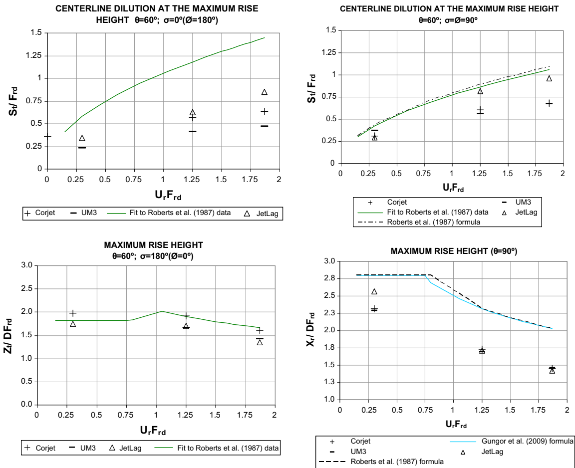
Fig. 8. Validation of centerline dilution at the maximum height for dense jets, for different \theta - \phi combinations (dynamic environment).
