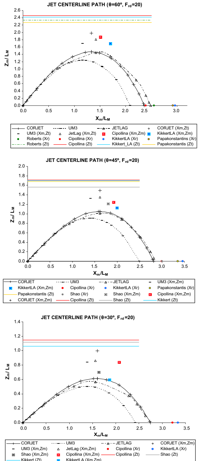
Fig. 6. Horizontal location and minimum dilution at the impact point.
