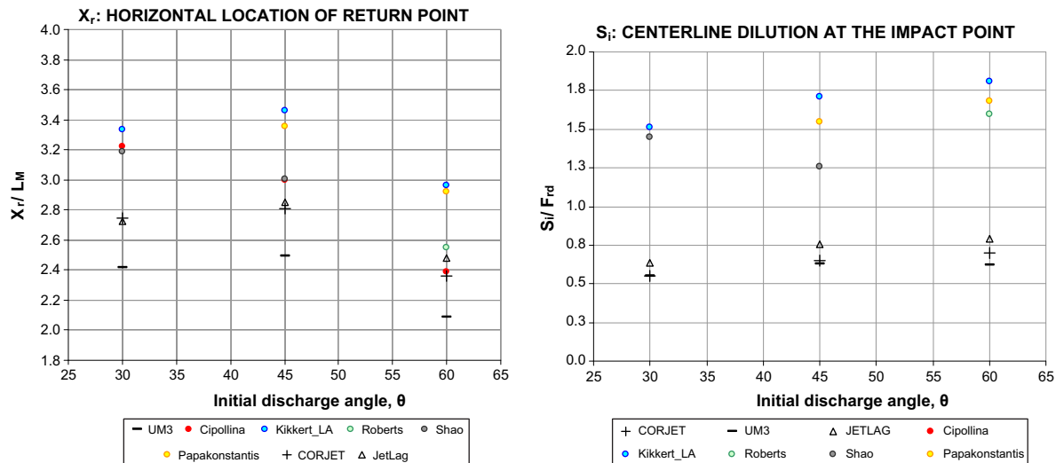
Fig. 5. Validation of return point dilution for inclined dense jets (stagnant ambient).
