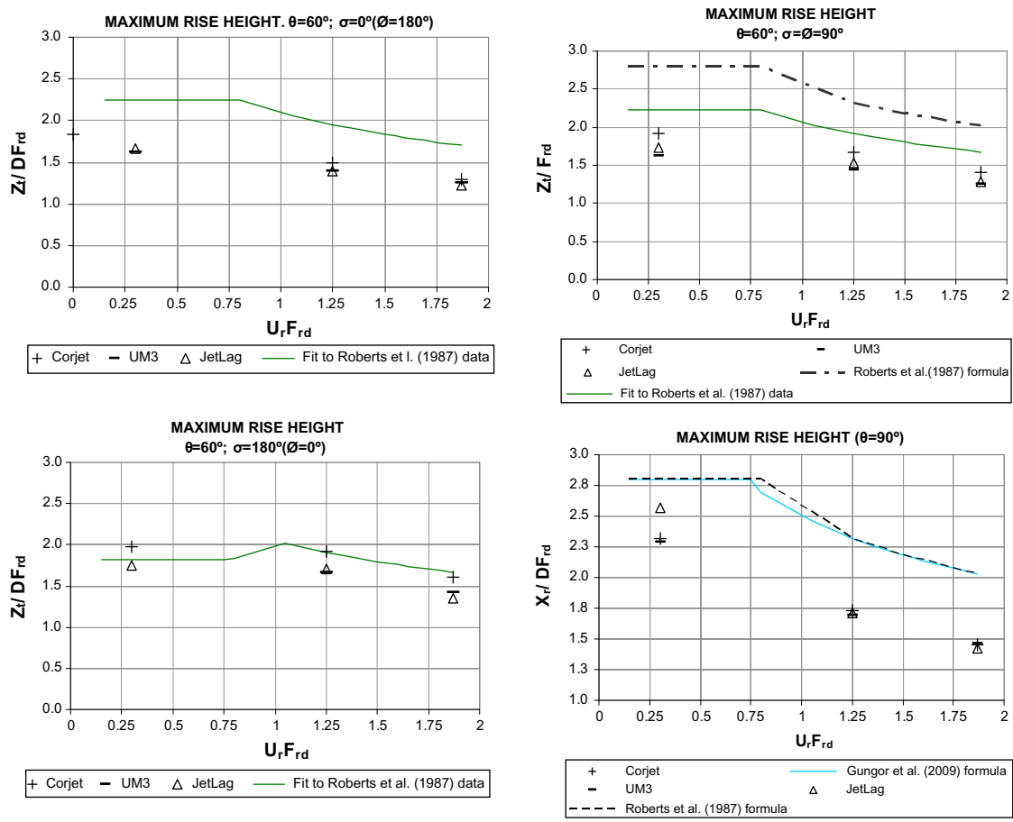
Fig. 7. Validation of maximum rise height for dense jets, for different \theta - \phi combinations (dynamic environment).
