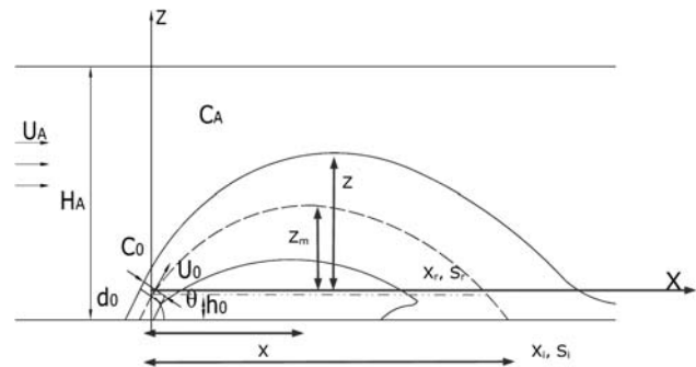
Fig. 2. Profile view of an inclined dense jet. Where H_A : average depth at discharge point; U_A : ambient velocity; C_A : ambient salinity; \rho_A : Ambient density; \sigma : horizontal angle between jet and current; \phi : angle of crossflow to the vertical plane containing the nozzle axis \phi = 180^\circ - \sigma ; U_o : initial discharge velocity; \rho_o : effluent density; C_o : effluent salinity concentration; h_o : port height; d_o = D : port diameter; and \theta : jet discharge angle (vertical angle with respect to the bottom).
