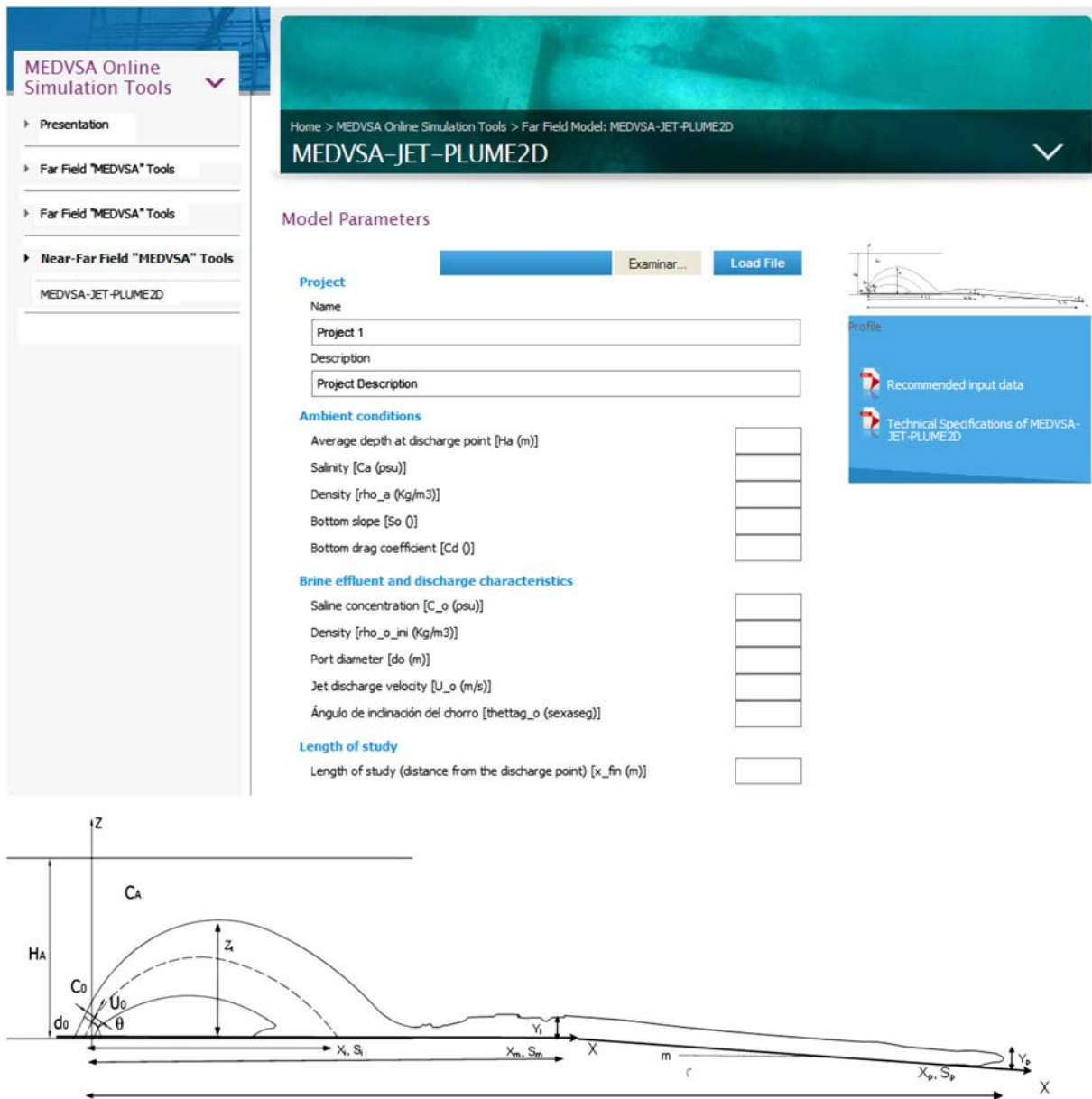
Fig. 10. Interface of the model MEDVSA-JET-PLUME2D and scheme of the jet path, spreading layer and hypersaline plume modeled.
