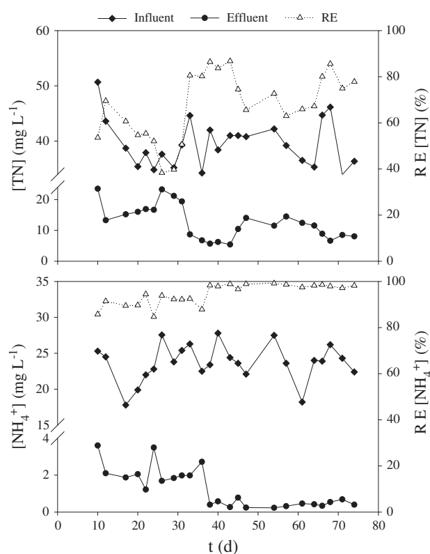
Fig. 4. Influent/effluent concentrations and RE of TN and \text{NH}_4^+ during the experimental campaign.
