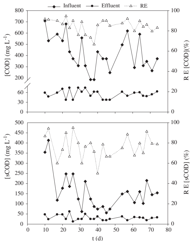
Fig. 2. Influent/effluent concentrations and RE of COD and sCOD during the experimental campaign.
