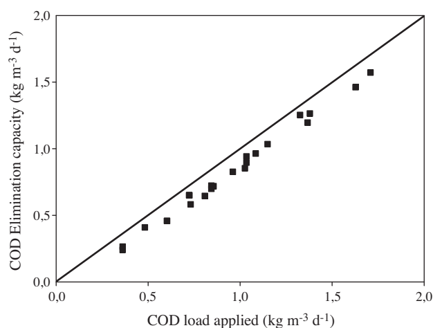
Fig. 3. Organic load applied versus elimination capacity in terms of COD (the axes' bisector line representing the theoretical 100% removal).
