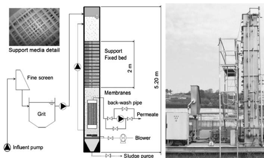
Fig. 1. Diagram and picture of the demonstrative plant configuration and main components with a detail of the BLAS [16] fixed bed support media (top, left side) inside the reactor.
