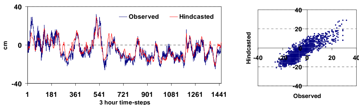
Fig. 3. Observed (Bilbao tide gauge) and hindcasted (SIMAR 44) time series (left) and scatterplot (right) of meteorological sea level residuals (measured sea level minus astronomical tide). Temporal resolution: 3 h (00:00, 03:00, 06:00, 09:00, 12:00, 15:00, 18:00 and 21:00 UTC) time steps from 1 October 1992 to 31 March 1993.
