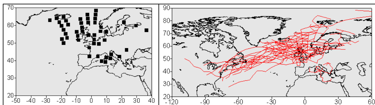
Fig. 9. Location of the storm pressure minimum and corresponding storm tracks for independent eTWL events along the coast of northern Spain derived from instrumental data (1992–2008).
