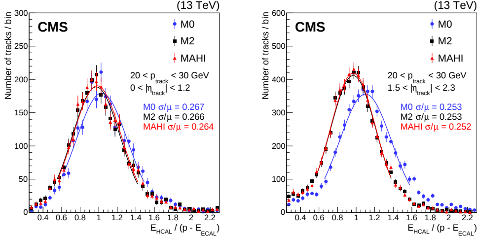
Figure 6. The HCAL energy response of M0, M2, and MAHI, measured in an electron/photon-triggered data set using isolated tracks with 20 < p_{\text{track}} < 30 \text{ GeV} and either |\eta_{\text{track}}| < 1.2 (left) or 1.5 < |\eta_{\text{track}}| < 2.3 (right). The vertical bars show the statistical uncertainty in the number of tracks in each bin. The measured energy resolution for each method in this sample is comparable.
