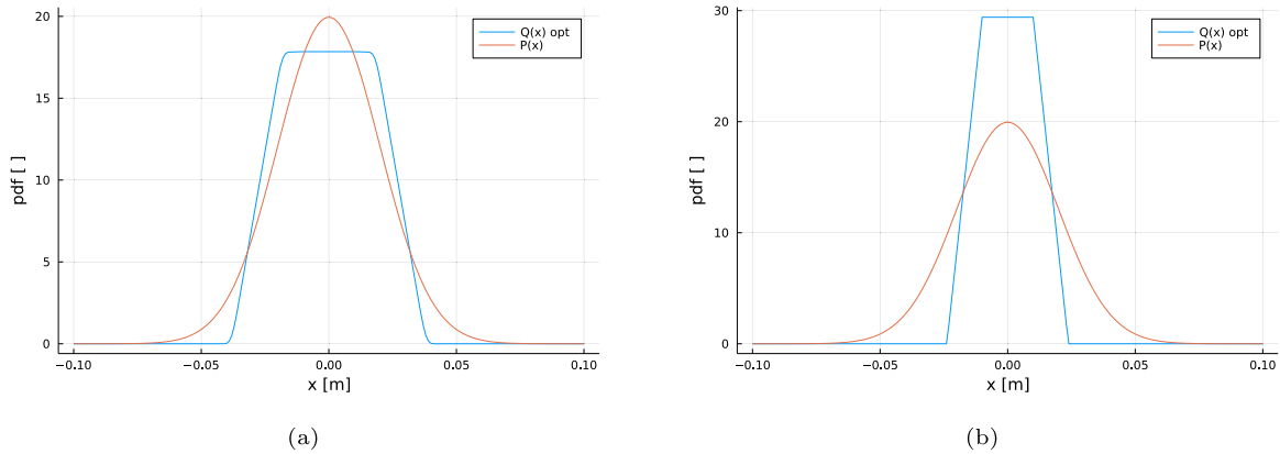
Fig. 32. Two different optimized beam-line distributions Q(x) for n = 3 apertures. (a) uses only D_{KL} and \mathcal{L}_2 , enforcing a good distribution approximation of P(x) with equally sized apertures; (b) utilizes \mathcal{L} as in Eq. (29), sacrificing function approximation quality for lower background levels.
