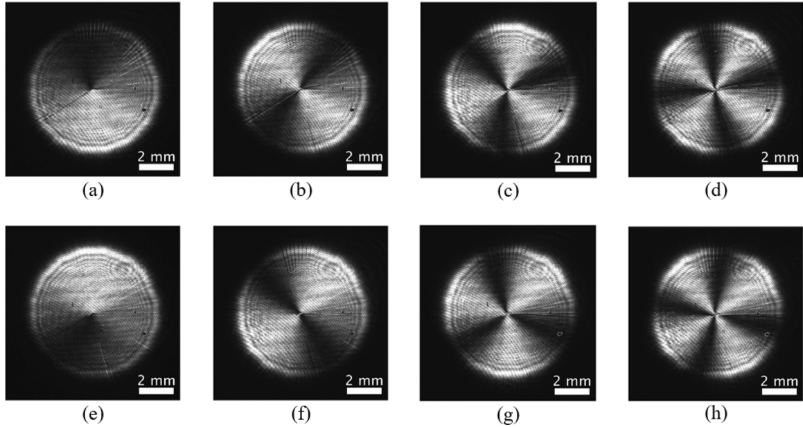
Fig. 5. Phase shift for different topological charges (a) l = 1 , V_1 = 1.6 V RMS , V_2 = 1.46 V RMS , (b) l = 2 , V_1 = 1.6 V RMS , V_2 = 1.34 V RMS , (c) l = 3 , V_1 = 1.61 V RMS , V_2 = 1.24 V RMS , (d) l = 4 , V_1 = 1.61 V RMS , V_2 = 1.14 V RMS . (e)–(h) For l = -1 to l = -4 the inverted voltages in V_1 and V_2 are applied.
