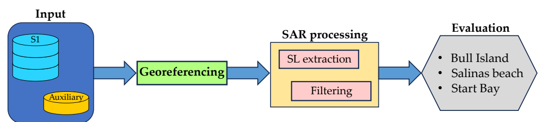
Figure 1. Overall methodology used to assess shoreline change from SAR satellite imagery in three macro-tidal coastal environments. SAR-S1 data, combined with auxiliary data, are used to extract SAR-SLs, distances from the reference line (RL), and annual change rates. Interpretation of SAR-SLs is performed for three different locations.
