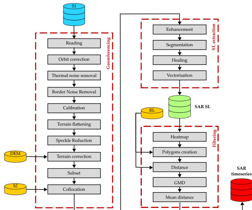
Figure 4. SAR processing flowchart used in this study showing the three main consecutive steps of georeferencing, SL extraction, and filtering.
