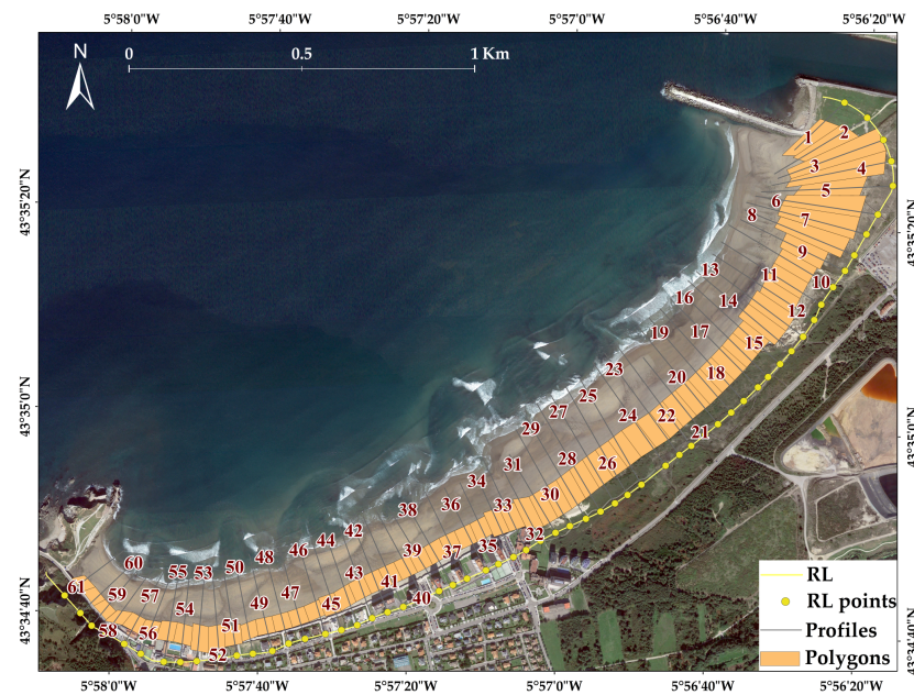
Figure 7. SAR polygons and beach profiles, indicated by numbers, for Salinas beach. Source of aerial imagery: Esri, World Imagery Metadata.
