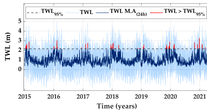
Figure A3. Total water level (TWL) time series and moving average (M.A.) based on a 24 h sampling window.
