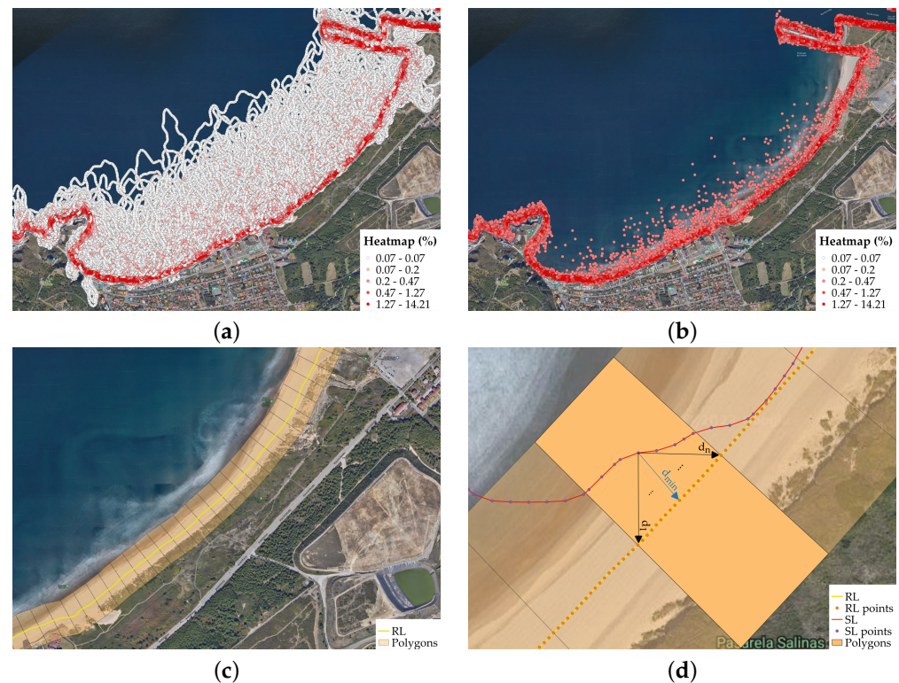
Figure 5. Shoreline filtering for Salinas beach: (a) heatmap distribution considering all SL points; (b) points following an initial filtering process, revealing a distinct and clear SL pattern; (c) polygon creation; (d) distance between each SL point and the RL (b). Source of aerial imagery: Google, ©2023 Maxar Technologies.
