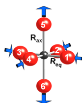
Figure 1. Description of a tetragonally elongated \text{CuF}_6^{4-} complex.
