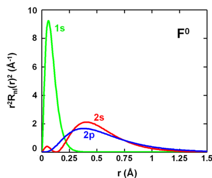
Figure 2. Radial probability densities P_j(r) = r^2 R_j^2(r) ( j = 1s, 2s, 2p ) corresponding to free fluorine atom calculated by means of the atomic wavefunctions of Bunge et al. 29
