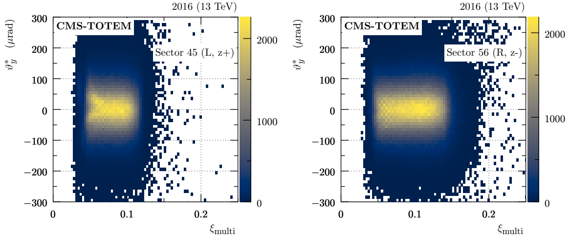
Figure 26. Histogram of \theta_y^* vs. \xi as reconstructed with the multi-RP method (fill 5276, 2016). The color code represents per-bin event counts. Left: sector 45, right: sector 56.
