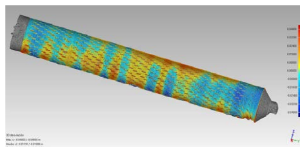
Fig. 7. Deformation Chart between real and theoretical industrial hopper.
