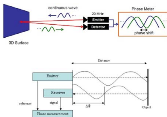
Fig. 1. Outline of operations of a laser phase difference scanner [12].
