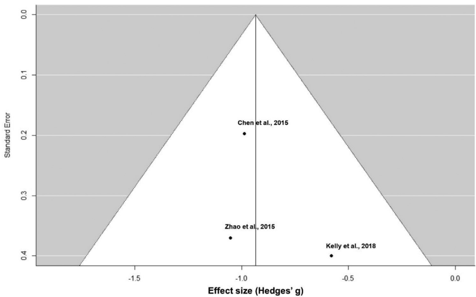
Fig. 4. Funnel plot of the sensitivity meta-analysis of placebo-controlled RCTs for prolactin reduction.
