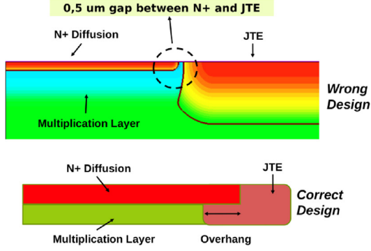
Fig. 6. 2D Numerical simulation at the pad peripheral area of the LGAD. The gap between N^+ and JTE diffusion was found to reproduce the high leakage current problem experimentally observed. The problem was mitigated by introducing an overhang of the N^+ into the JTE diffusion.
