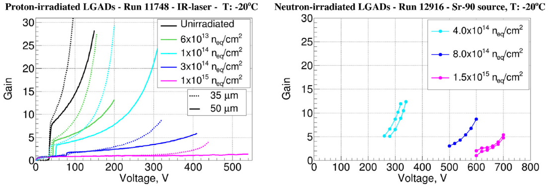
Fig. 12. Gain measurements after irradiation. The gain was evaluated according to the expression (3). A gain degradation with fluence is observed (more severe in the case of protons) and a higher gain degradation of the 50 μm LGADs with respect to the 35 μm ones can be seen.
