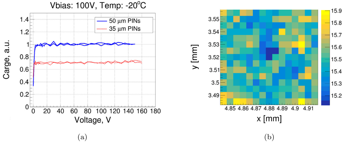
Fig. 11. (a) Comparison between PINs charge collection from wafers W5 and W11. (b) Gain surface homogeneity in one of the unirradiated LGADs from wafer W11.
