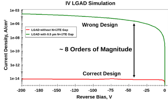
Fig. 6. 2D Numerical simulation at the pad peripheral area of the LGAD. The gap between N^+ and JTE diffusion was found to reproduce the high leakage current problem experimentally observed. The problem was mitigated by introducing an overhang of the N^+ into the JTE diffusion.
