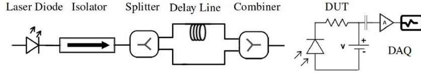
Fig. 17. Timing setup schematic with all its main components: laser diode, isolator, splitter, delay line, combiner, and DUT.
