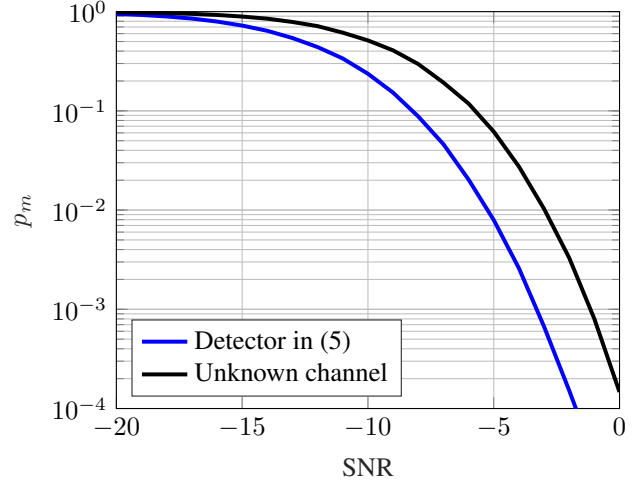
Fig. 2: Probability of missed detection vs. \text{SNR}_s = \text{SNR}_r = \text{SNR} for an experiment with N = 32 , L = 4 and p_{fa} = 10^{-4}
