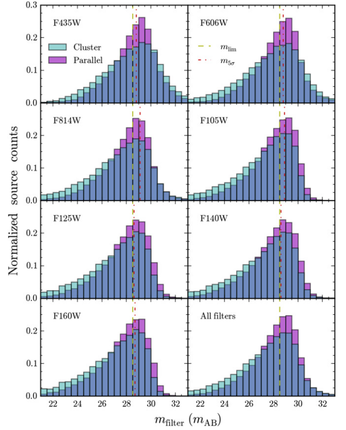
Figure 1. Normalized source counts (i.e., area under each histogram is equal to unity) in the 10 HFF C15 catalogs as a function of the apparent magnitude m_{\text{filter}} in individual HFF filters (labelled at the upper left corner of each panel). Cyan and magenta bars denote the source counts in the cluster and parallel fields respectively. Yellow dashed lines show the apparent magnitude limit m_{\text{lim}} = 28.5 that we set for all filters in subsequent analysis, whereas the red dashed-dotted lines show the expected 5\sigma point-source limiting magnitudes for the corresponding HFF filters. The bottom right panel shows the normalized total source counts irrespective of filter.
