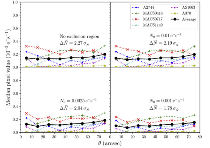
Figure 5. Same as Figure 4 for the parallel fields, where the “center” of each such control field was chosen to be approximately the center of the field of view. Note that the vertical scale is one dex lower than that of Figure 4, primarily because there is only little brightening of the sky background, if any, by diffuse light when compared to the cluster fields.
