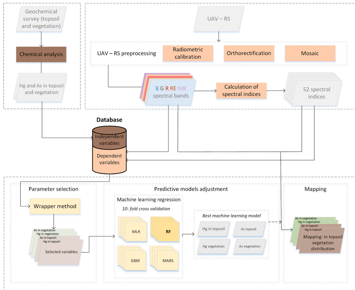
Fig. 1. Process workflow.
