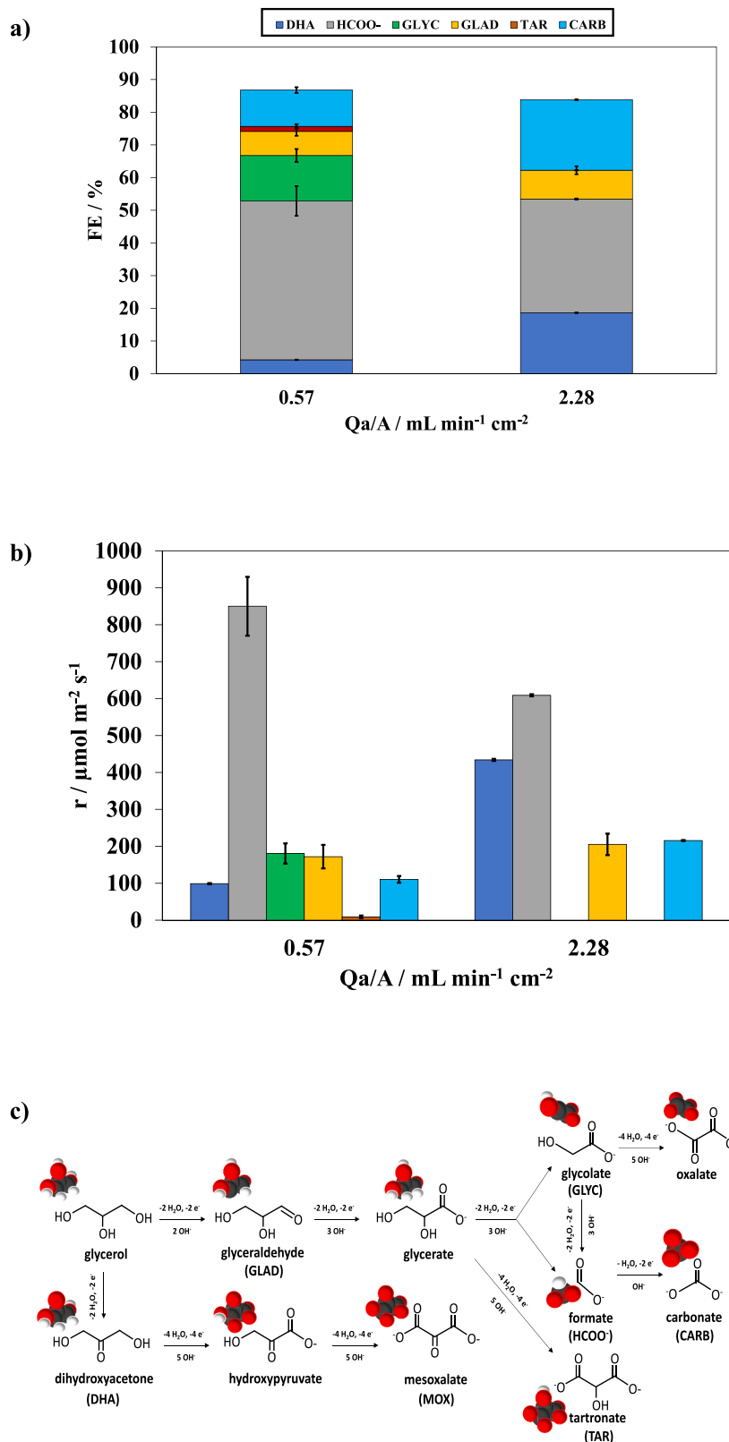
Fig. 3. a) Faradaic Efficiencies [FE] and b) production rates [r] of the different detected products from GOR in the gas-phase MEA reactor as a function of the anolyte flow rate per geometric anode surface area ( Q_a/A ) with a single-pass operation though the anode compartment at fixed values of the \text{H}_2\text{O}/\text{CO}_2 molar ratio per geometric cathode surface area and the current densities of 0.02 \text{ mol H}_2\text{O} [\text{mol CO}_2 \text{ cm}^2]^{-1} and 45 \text{ mA cm}^{-2} , respectively. c) Possible reaction pathways for the electrochemical oxidation of glycerol to various value-added products in alkaline medium. Adapted from ref. [43].
