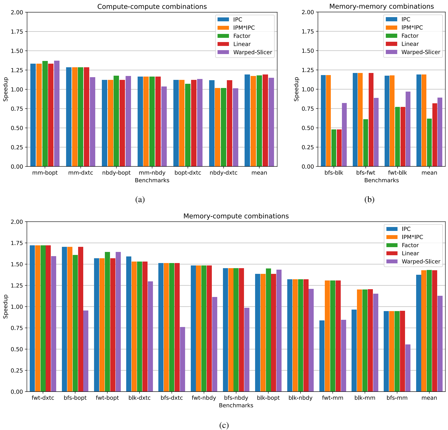
Figure 4.2: The speedup achieved by each algorithm relative to sequential execution of each pair of benchmarks. Per combination group mean values are plotted alongside.
