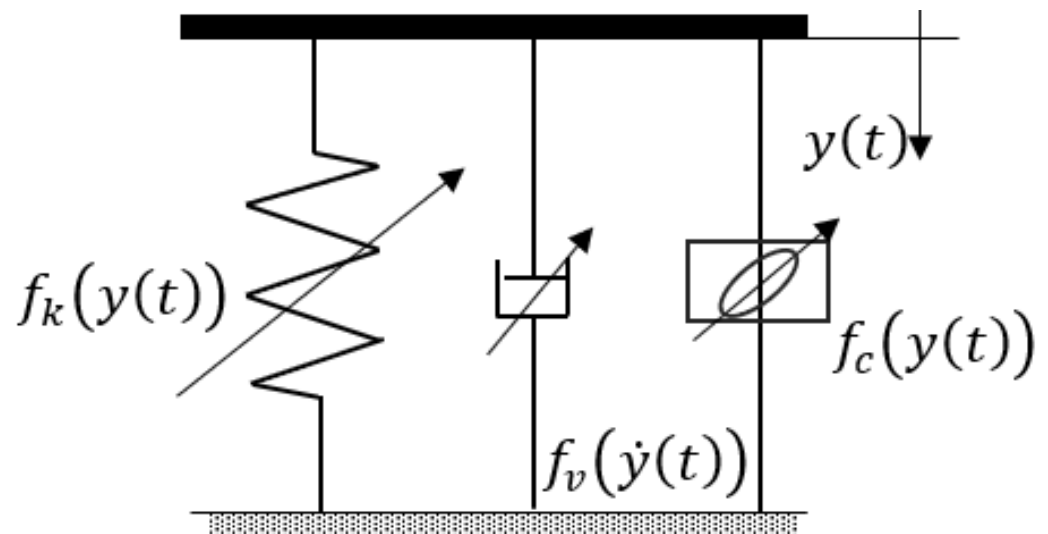
Figure 16. Mechanical model of the isolator.
