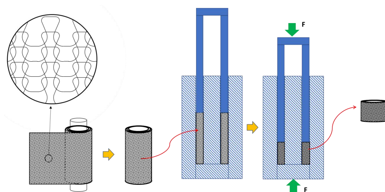
Figure 1. Steps of manufacturing process.
