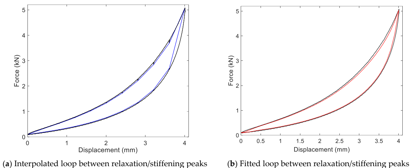
Figure 17. Hysteresis loops for testing with stops.
