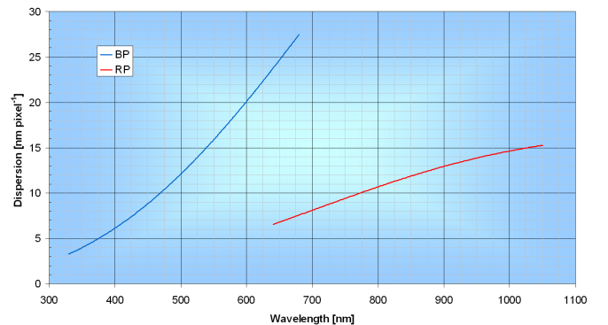
Fig. B.1. Nominal dispersion curves of the BP/RP instrument.
