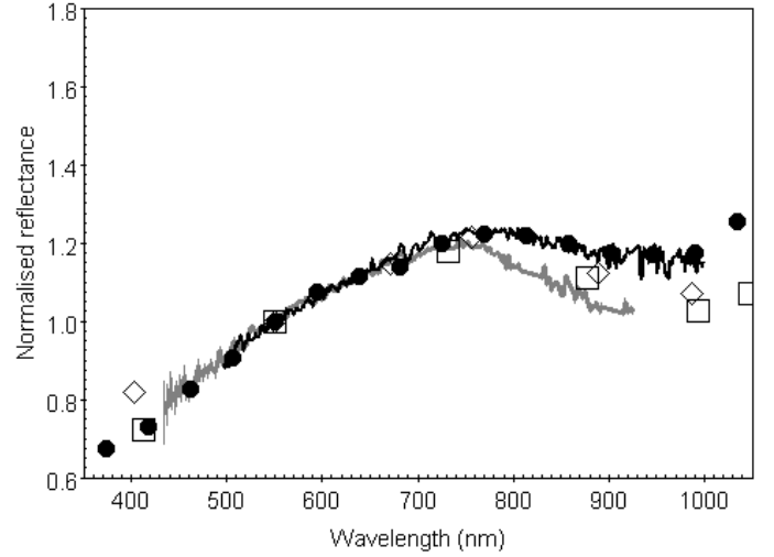
Fig. 18. Gaia mean reflectance spectrum of the asteroid (951) Gaspra, shown with black circles, together with literature ground-based spectra of Bus & Binzel (2002b) and Xu et al. (1995) with grey and black lines, respectively. Data obtained in space by NASA Galileo mission (Granahan et al. 1994) at phase angles of 51° and 31° are also shown with open squares and diamonds, respectively.
