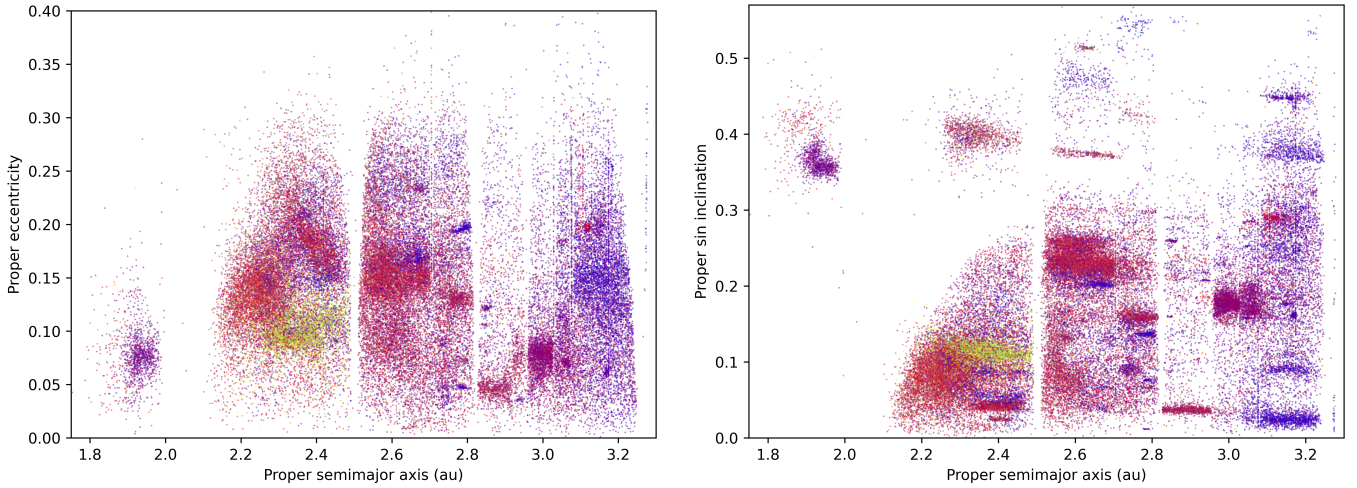
Fig. 12. Proper semi-major axis vs. proper eccentricity and sin of proper inclination for Gaia DR3 SSOs of the main-belt and Hungaria region. The colour of each dot is representative of the object's colour measured by Gaia according to the colour scheme defined in Sect. 4.2.
