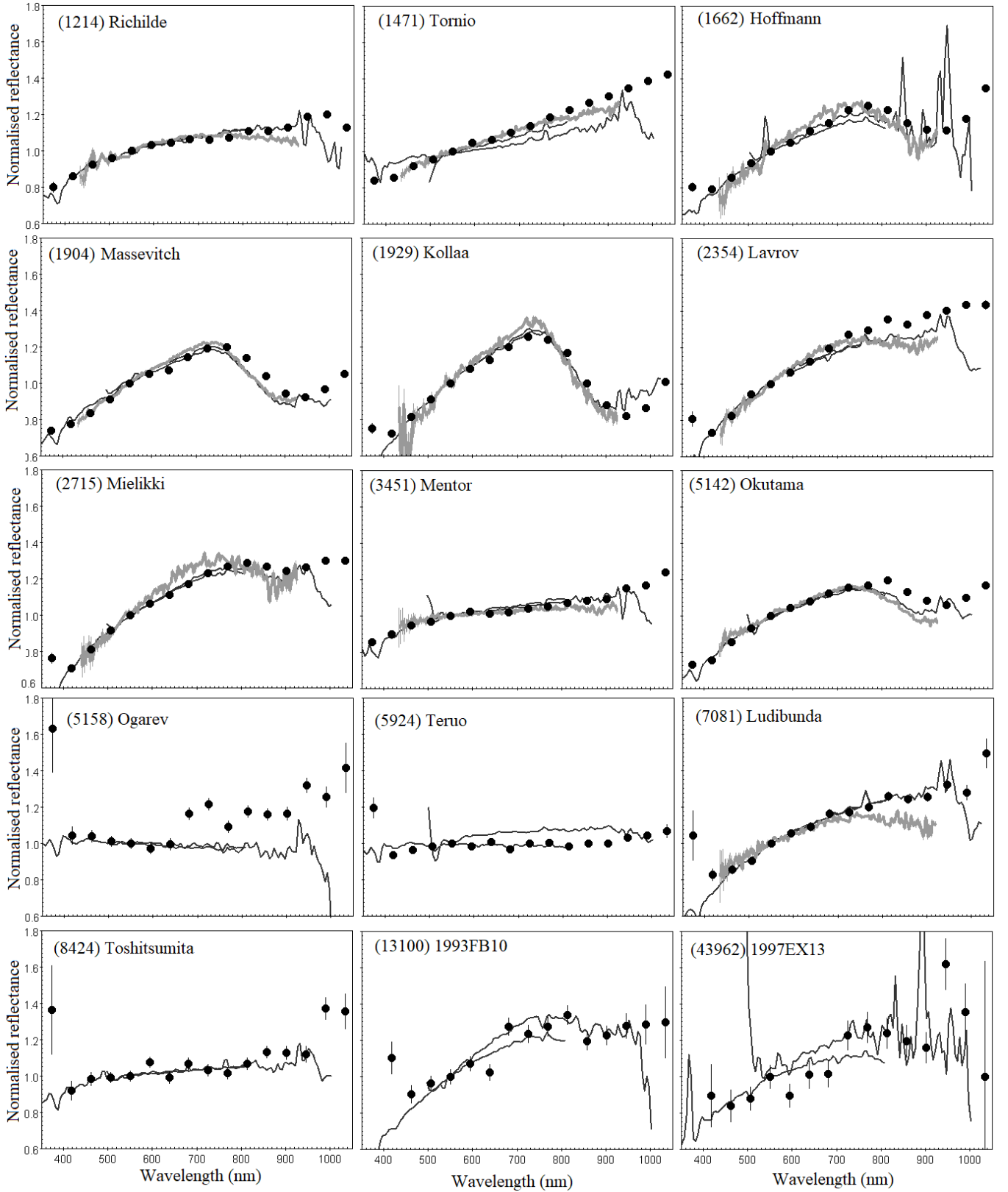
Fig. H.2. Gaia 's mean reflectance spectra (black circles) against ground-based observations; Cellino et al. (2020) spectra in dark grey lines and those of ( Bus & Binzel 2002b ) in light grey lines for asteroids (1214), (1471), (1662), (1904), (2354), (2715), (3451), (5142), (7081).
