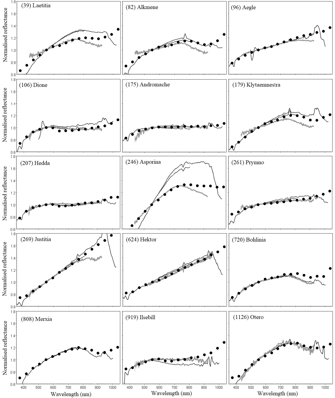
Fig. H.1. Gaia 's mean reflectance spectra (black circles) against ground-based observations; Cellino et al. (2020) spectra in dark grey lines and in light grey lines for asteroids (624) (Vilas et al. 1993) and (39), (82), (96), (106), (207), (246), (261), (269), (720), (919), (1126) (Bus & Binzel 2002b).
