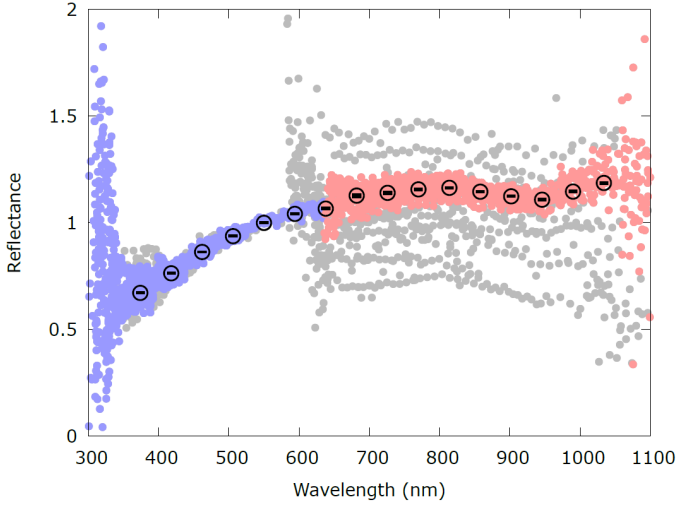
Fig. 5. Example of the mean computed reflectance \bar{R}(\lambda_i) (black circles) for the asteroid (61) Danae. The grey points are the R(\lambda_i)_t , corresponding to each epoch reflectance. The R(\lambda_i)_t values that are accepted by our filtering method are coloured in light blue (BP) and light red (RP).
