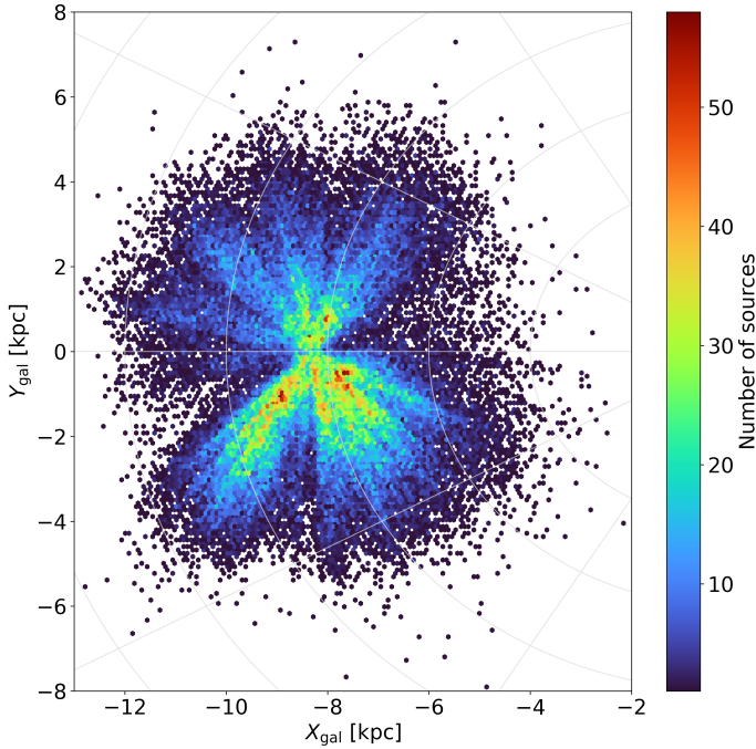
Fig. 3. Distribution of the Galactic sources of the dataset shown in Fig. 2, limited to those 71 490 stars with 0 < \sigma_\pi/\varpi \leq 0.25 , projected on the equatorial plane of the Galactocentric reference frame.
