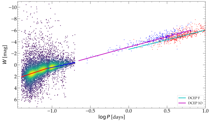
Fig. 13. Comparison between the PW relation(s) calculated in this paper for the fundamental F -mode \delta Sct (as in Fig. 12) and those of F - (red dots) and the first overtone IO-mode (blue dots) classical Cepheids. For the latter pulsators, the data and the PWs were taken from Poggio et al. (2021). For clarity, only objects with relative error on the photometric parallax better than 20% are plotted.
