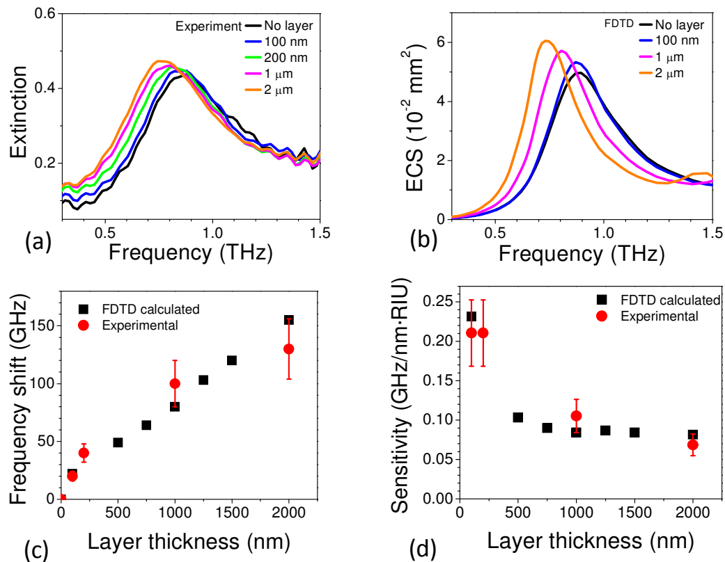
Fig. 2. a) Extinction, defined as (1 - \text{Transmission}) , of a collection of doped silicon bowtie antennas as a function of the thickness of the deposited \text{SiO}_2 layer; b) FDTD calculated extinction cross section (ECS) of an individual doped silicon bowtie antenna covered with \text{SiO}_2 layers of different thickness; c) Shift of the resonance frequency for the same situation as in a) and b) as a function of the top layer thickness, as obtained from experiments (red circles) and from FDTD calculations (black squares); d) Sensitivity of the bowtie antenna expressed in frequency shift per nanometer of film thickness, estimated from the experimental (red circles) and calculated (black squares) shift of the resonance.
