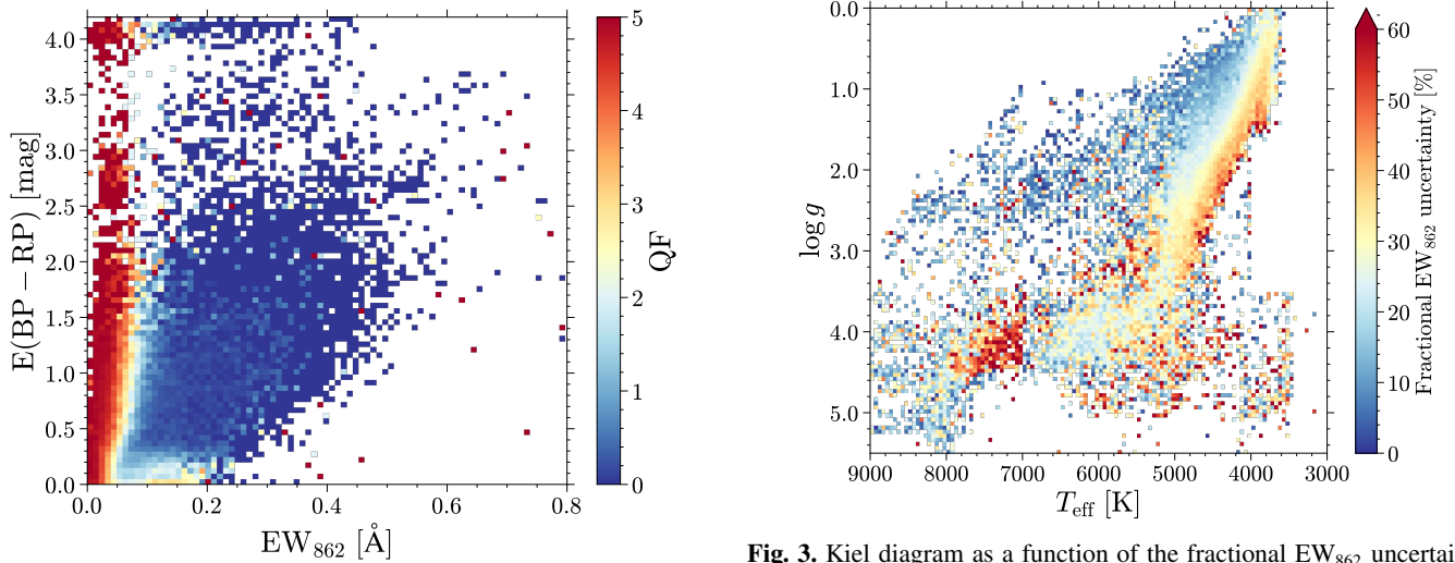
Fig. 2. Equivalent width vs. E(BP - RP) for the DIB \lambda 862 sample coloured by the mean QF calculated in 0.01 \text{ Å} \times 0.05 \text{ mag} bins.
