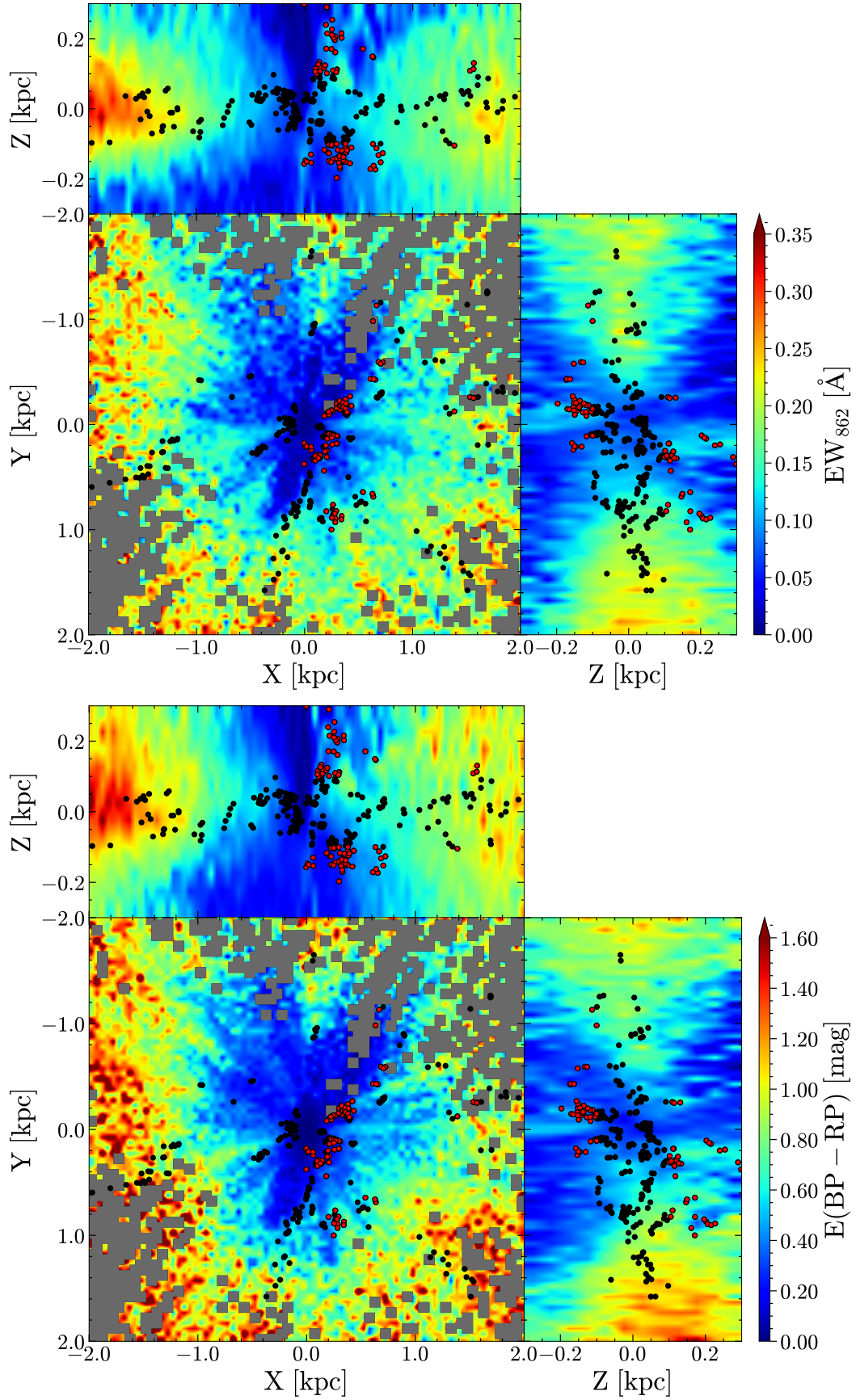
Fig. 13. Same as Fig. 11 but for a subsample containing 39 224 cases with |X| \leq 2 kpc, |Y| \leq 2 kpc, |Z| \leq 0.3 kpc, and valid E(BP - RP) . Median EW_{862} are taken from 0.05 \text{ kpc} \times 0.05 \text{ kpc} bins in XY , XZ , and YZ planes, respectively. Overplotted are nearby MCs measured in Zucker et al. (2020). The MCs with Z \geq 0.1 kpc are indicated as red dots.
