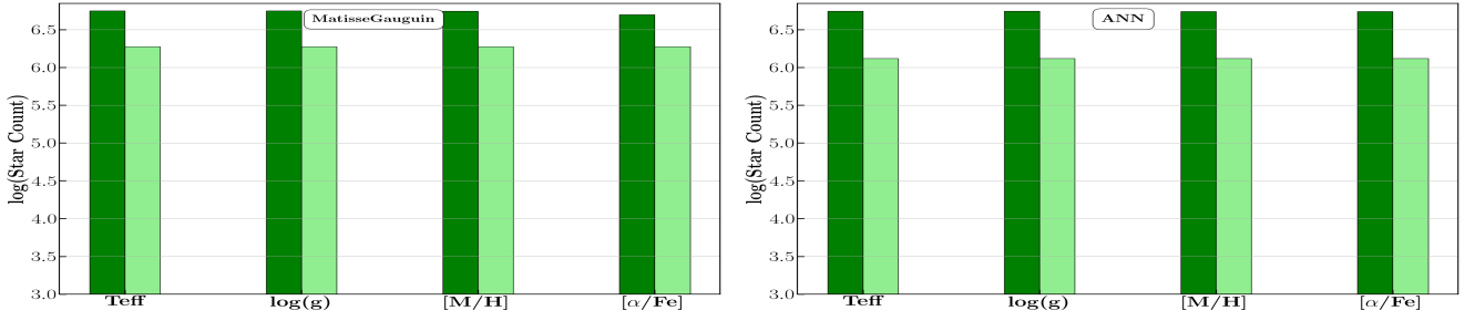
Fig. 17. Number of stars whose atmospheric parameters have been derived by MatisseGauguin and ANN ( left and right panels , respectively). The dark green histograms refer to the whole sample whereas the light-green ones show only the very best parametrised stars with all their parameter quality flags equal to zero.
