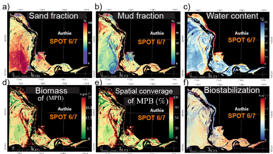
Fig. 7 Maps representing a sand and b mud, c water contents in %, d MPB biomass (mg.m -2 ) spatial coverage of biofilm and biostabilization (N.m -2 ) at low tide from SPOT 6/7 image in the Authie bay in the Northern France
