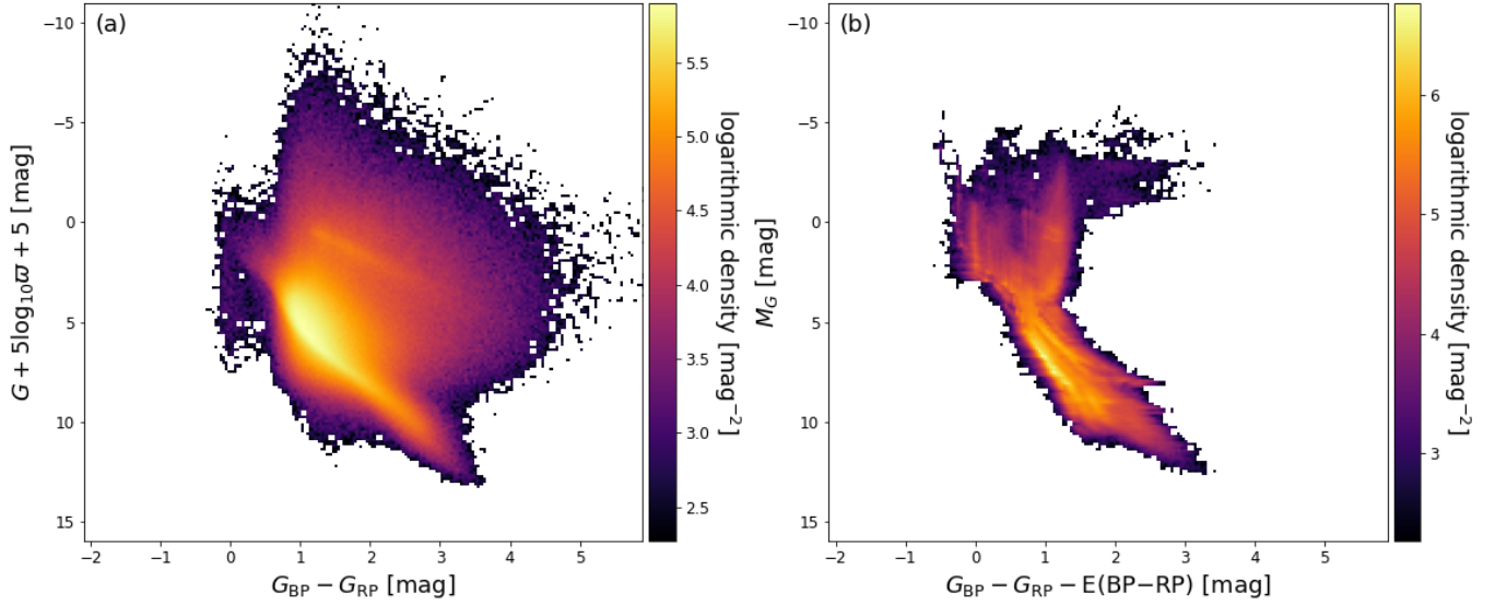
Fig. 4. Observed colour–magnitude diagram ( panel (a) ) and de-reddened colour–magnitude diagram ( panel (b) ). Both panels use the same sample of 2 598 519 stars that has been randomly selected from the main catalogue (see Appendix B for the ADQL query).
