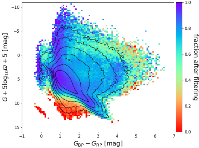
Fig. 2. Fraction of sources surviving the filtering described in Sect. 3.3 in the observed CMD. Contours indicate density of all sources with G \leq 19 . This figure used a random subset of 2815418 sources drawn from the main catalogue. This plot does not include sources without parallax measurement or with negative parallax.
