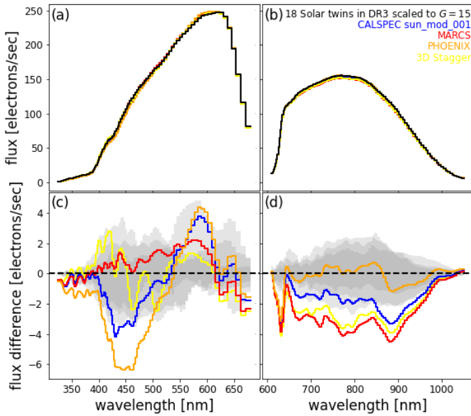
Fig. 1. Mismatch between observed BP/RP spectra of 18 solar twins from Galarza et al. (2021) with A_0 < 0.001 mag (black lines and grey contours) and model BP/RP spectra from PHOENIX (orange lines), MARCS (red lines), CALSPEC sun_model_001 (blue lines), and 3D Stagger (yellow lines). Panel (a): all BP spectra scaled to G = 15 . Panel (b): same as panel (a) but for RP. Panel (c): differences from median observed BP spectrum in panel (a). Panel (d): same as panel (c) but for RP. Grey contours in panels (c) and (d) indicate the pixel-wise central 68%, 90%, and min/max intervals given the 18 solar twins.
