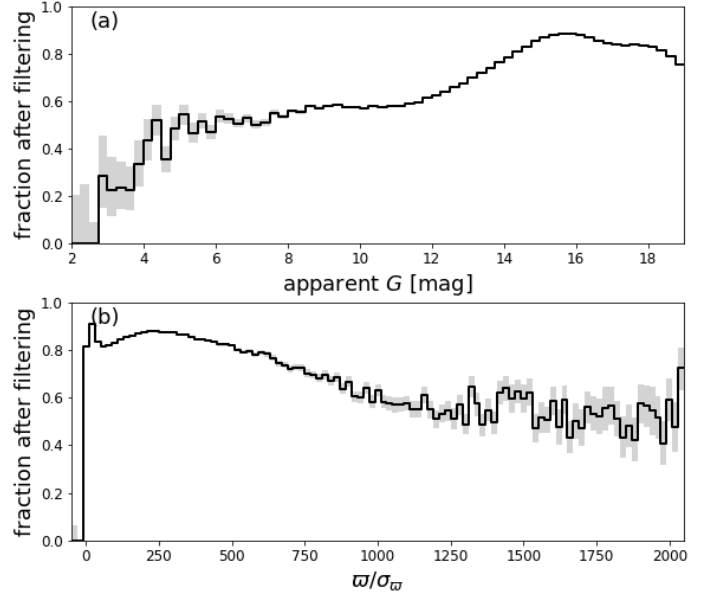
Fig. 3. Fraction of sources surviving the filtering described in Sect. 3.3 as a function of apparent G magnitude (panel (a)) and parallax signal-to-noise ratio (panel (b)). Both panels use a random subset of about 100 million sources with G < 19 . Grey intervals indicate the horizontally decreasing intervals of 68% confidence assuming a beta distribution in each bin.
