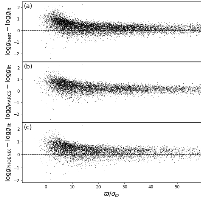
Fig. 9. Bias of surface gravity estimates for stars with low parallax signal-to-noise ratio, w/\sigma_w , for 25 169 red clump stars (Jönsson et al. 2020; Bovy et al. 2014). Panel (a): GSP-Phot best-library results. Panel (b): GSP-Phot MARCS library results. Panel (c): GSP-Phot PHOENIX library results.
