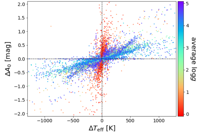
Fig. 19. Illustration of the temperature–extinction degeneracy using the parameter differences between pairs from the BP/RP split-epoch validation dataset (cf. Sect. 3.9). Colour-coding is done by the average surface gravity of both components.
