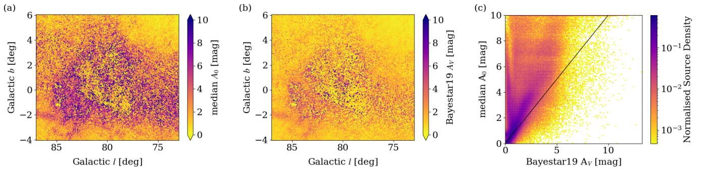
Fig. 15. Same as Fig. 14 but for the dense star-formation region Cygnus X1.
