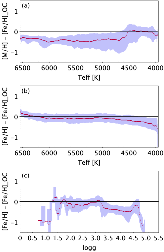
Fig. 11. Difference between GSP-Phot metallicities of individual FGK members and the mean [\text{Fe}/\text{H}] of the parent open cluster for stars with \frac{\sigma}{\sigma_{\text{eff}}} \geq 10 and MARCS models, before and after the calibration. We note that the calibration on LAMOST [\text{Fe}/\text{H}] values translates [\text{M}/\text{H}] to [\text{Fe}/\text{H}] . The red line is the median of the distribution. The blue area is delimited by the 16th and 84th quantiles. Panel (a): residuals versus T_{\text{eff}} before the calibration. Panel (b): residuals versus T_{\text{eff}} after the calibration. Panel (c): residuals versus \log g after the calibration.
