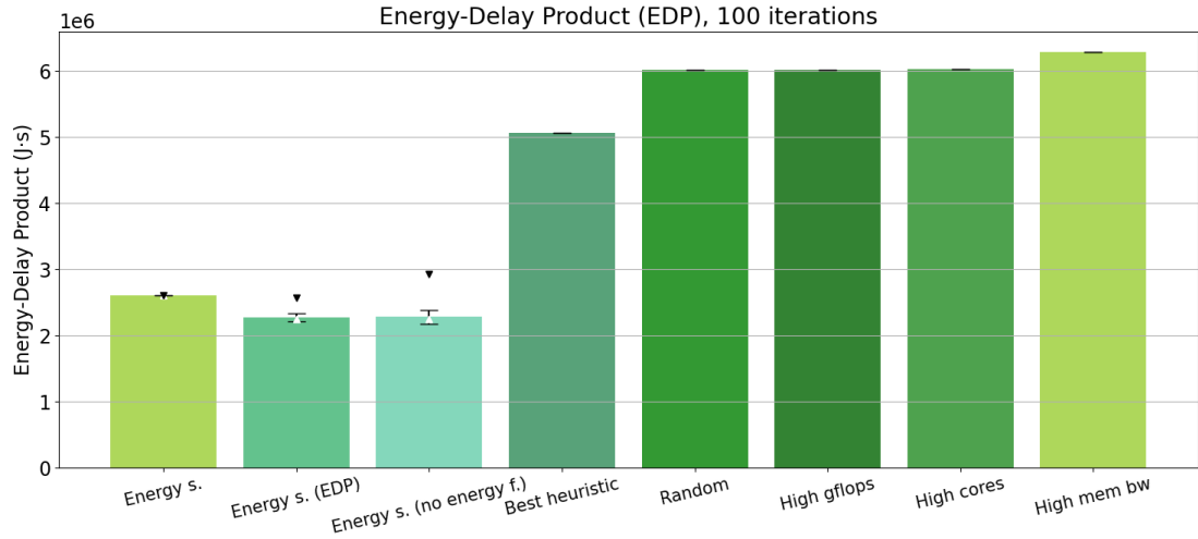
Figure 4.19: Experiment 2 - EDP comparison.
