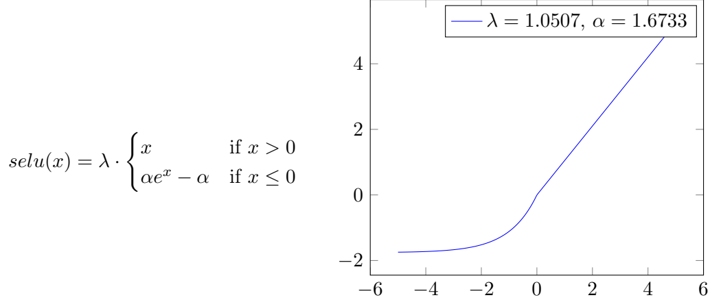
Figure 3.2: selu , the SELU activation function.
