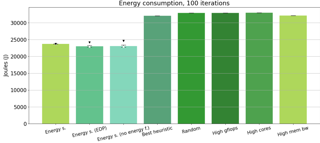
Figure 4.18: Experiment 2 - Energy consumption comparison.
