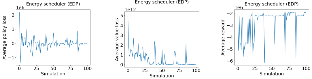
Figure 4.16: Experiment 2 - Loss and reward plots for the EDP objective.
