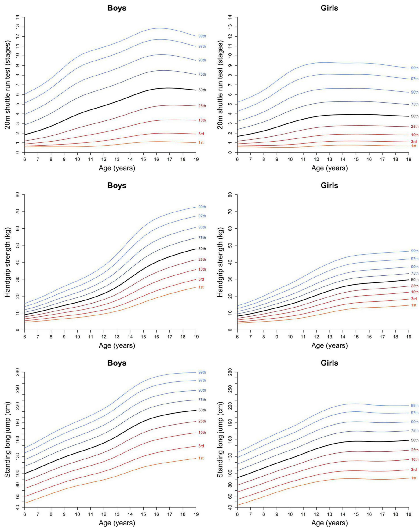
Figure 1 Percentile curves for cardiorespiratory and muscular strength tests among European children and adolescents. Smoothed percentiles were calculated using the generalised additive model for location, scale and shape method, and weights were applied according to country population. Data sources are available online ( https://www.fitbackeurope.eu/en-us/fitness-map/sources ) and in online supplemental table 1.
