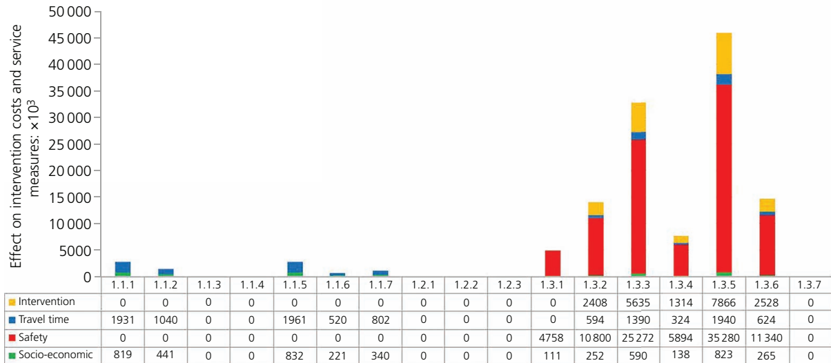
Figure 2. Infrastructure: measures of resilience for each indicator, using the actual value of all indicators, by intervention costs and each measure of service
