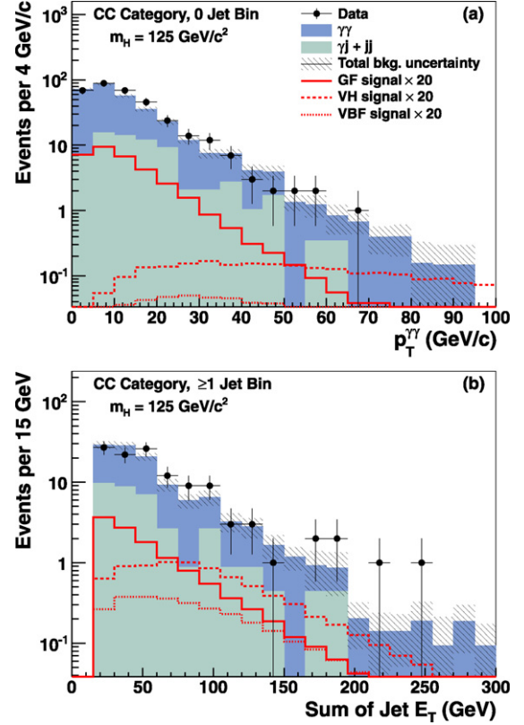
Fig. 3. For a Higgs boson mass of 125 \text{ GeV}/c^2 , a comparison of the data to the background prediction in (a) the p_T^{\gamma\gamma} distribution for the CC0 category and (b) the distribution of the sum of the reconstructed jet E_T for the CCJ category. The expected SM Higgs boson signal for the three production processes is multiplied by a factor of 20.
