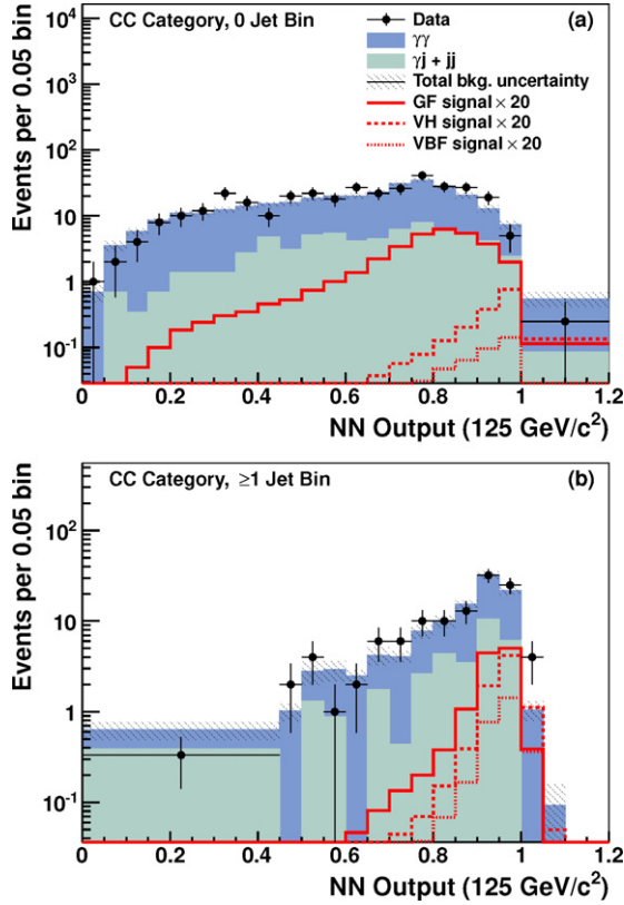
Fig. 4. For a Higgs boson mass of 125 GeV/c 2 , a comparison of the NN output distributions for the data and the background prediction for (a) the CC0 category and (b) the CCJ category. The expected SM Higgs boson signal for the three production processes is multiplied by a factor of 20.
