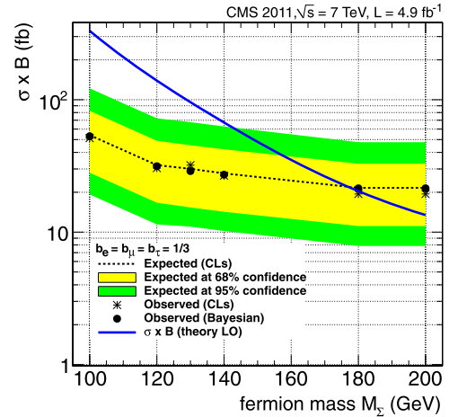
Fig. 3. The expected (dashed line) and observed (asterisks and black points) exclusion limits at 95% confidence level on \sigma B as a function of the fermion mass M_\Sigma , assuming b_e = b_\mu = b_\tau = 1/3 (FDS) for the signal. The solid (blue) curve represents the predictions of the LO type III seesaw models. The light (yellow) and dark (green) shaded areas represent, respectively, the 1 standard deviation (68% CL) and 2 standard deviations (95% CL) limits on the expected results obtained from MC pseudo-experiments, which reflect the combined statistical and systematic uncertainties of the SM contributions. The asterisks and the black points show, respectively, the observed limits computed following a frequentist method based on the CLs criterion and a Bayesian approach.
