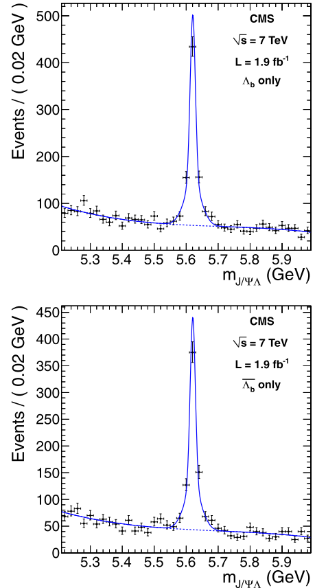
Fig. 1. Fit results for the m_{J/\psi\Lambda} distribution for \Lambda_b (top) and \bar{\Lambda}_b (bottom) for p_T^{\Lambda_b} > 10 \text{ GeV} and |y^{\Lambda_b}| < 2.0 , where the dashed line shows the background fit function, the solid line shows the sum of signal and background, and the points indicate the data.
