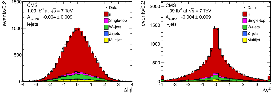
Fig. 2. Reconstructed \Delta|\eta| (left) and \Delta y^2 (right) distributions for the combined lepton + jets channel. The last bins include the sum of all contributions for |\Delta|\eta|| > 4.0 and |\Delta y^2| > 4.0 , respectively. The signal and background contributions are normalized to the results in Table 1.
